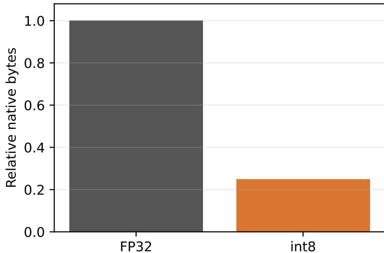
int8 RMSE 0.0103
