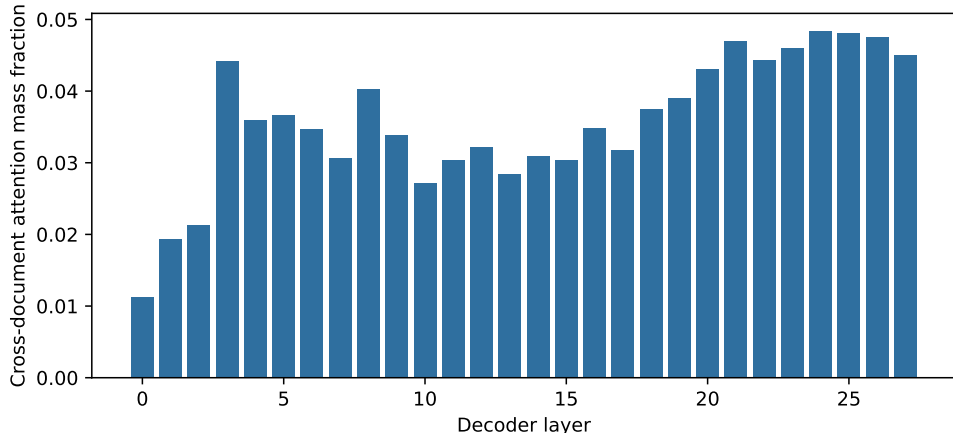
Figure 3: Mean share of packed-teacher cross-document attention mass by decoder layer. Later layers carry more aggregate mass, but no narrow layer band dominates.
