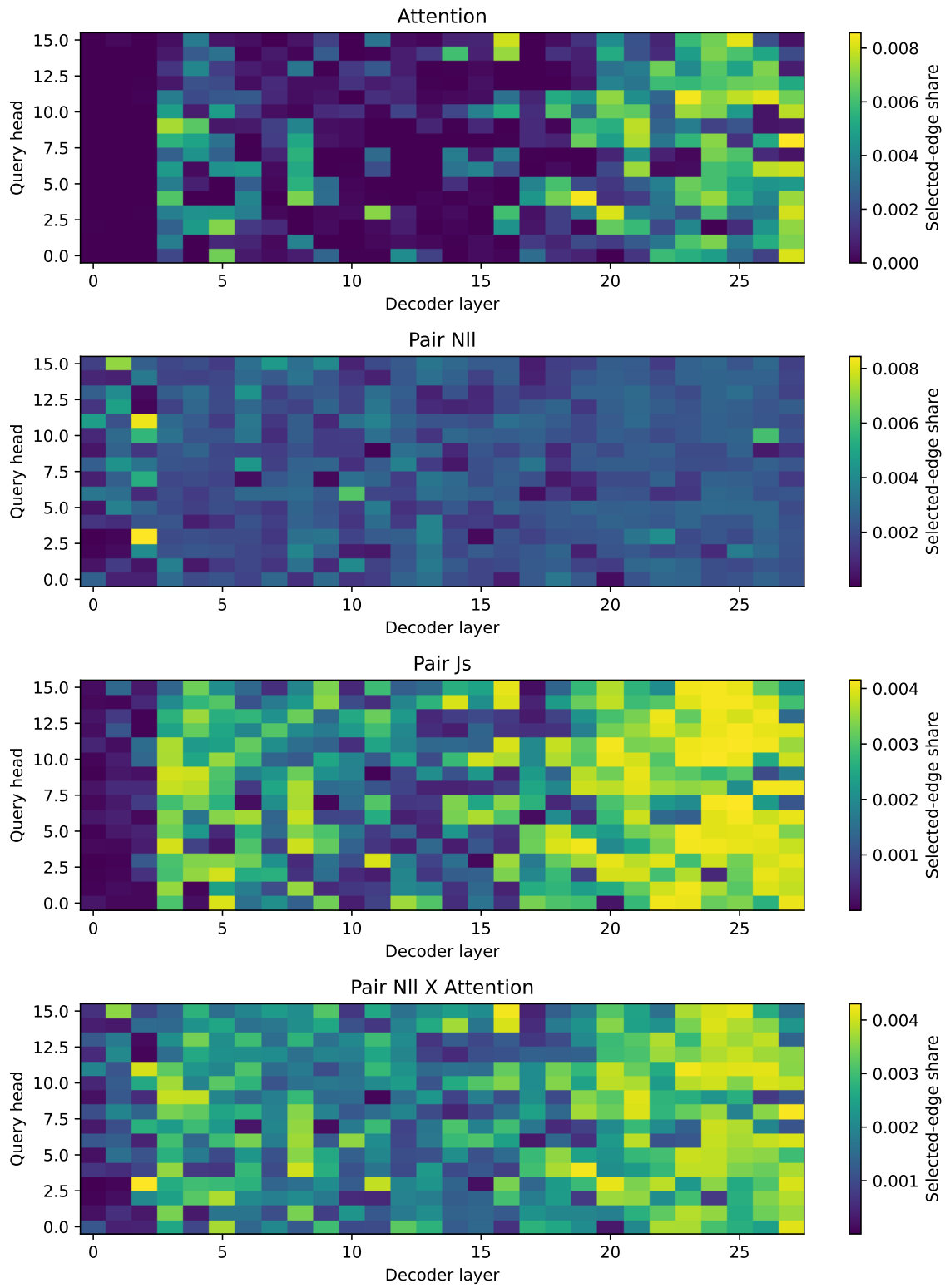
Figure 5: Layer-head allocation of each .1% plan over 150 frozen test questions. Color is selected-edge share within a policy.
