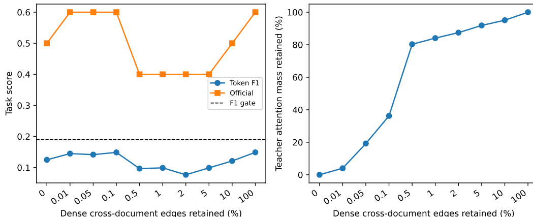
Figure 2: Task quality and retained teacher mass across physical top-edge budgets. The curve is a mechanism smoke over ten questions; connecting lines do not imply monotonicity or statistical precision.
