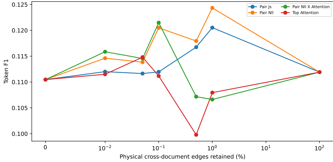
Figure 4: Powered-test F1 frontiers for observational and interventional rankings. Causal pair rankings improve the mean sparse frontier, but all curves remain non-monotonic; lines aid reading and do not imply interpolation.
