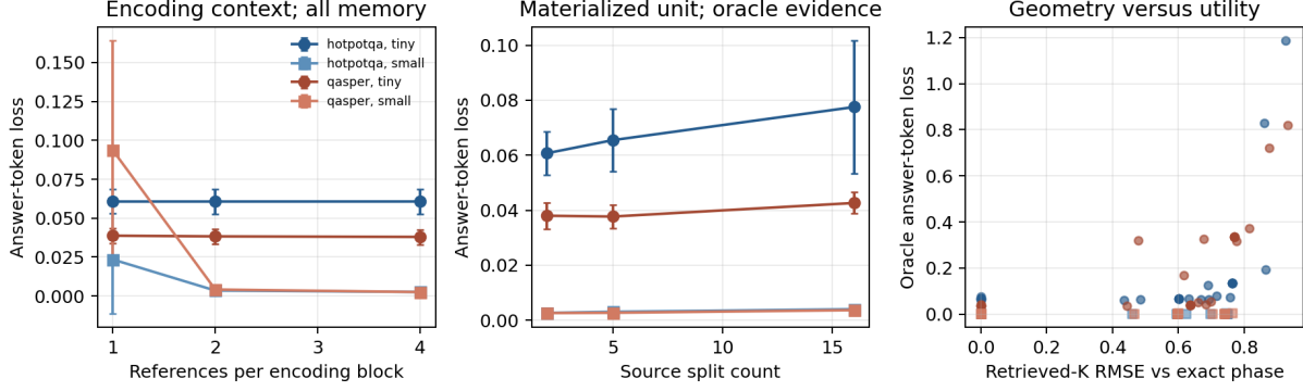
Figure 3: Left: larger encoding groups help when the resulting neighboring K/V is retained. Center: finer source partitioning generally raises oracle loss. Right: larger deviation from exact RoPE phase does not map monotonically to task loss. Error bars show one standard deviation over five seeds.
