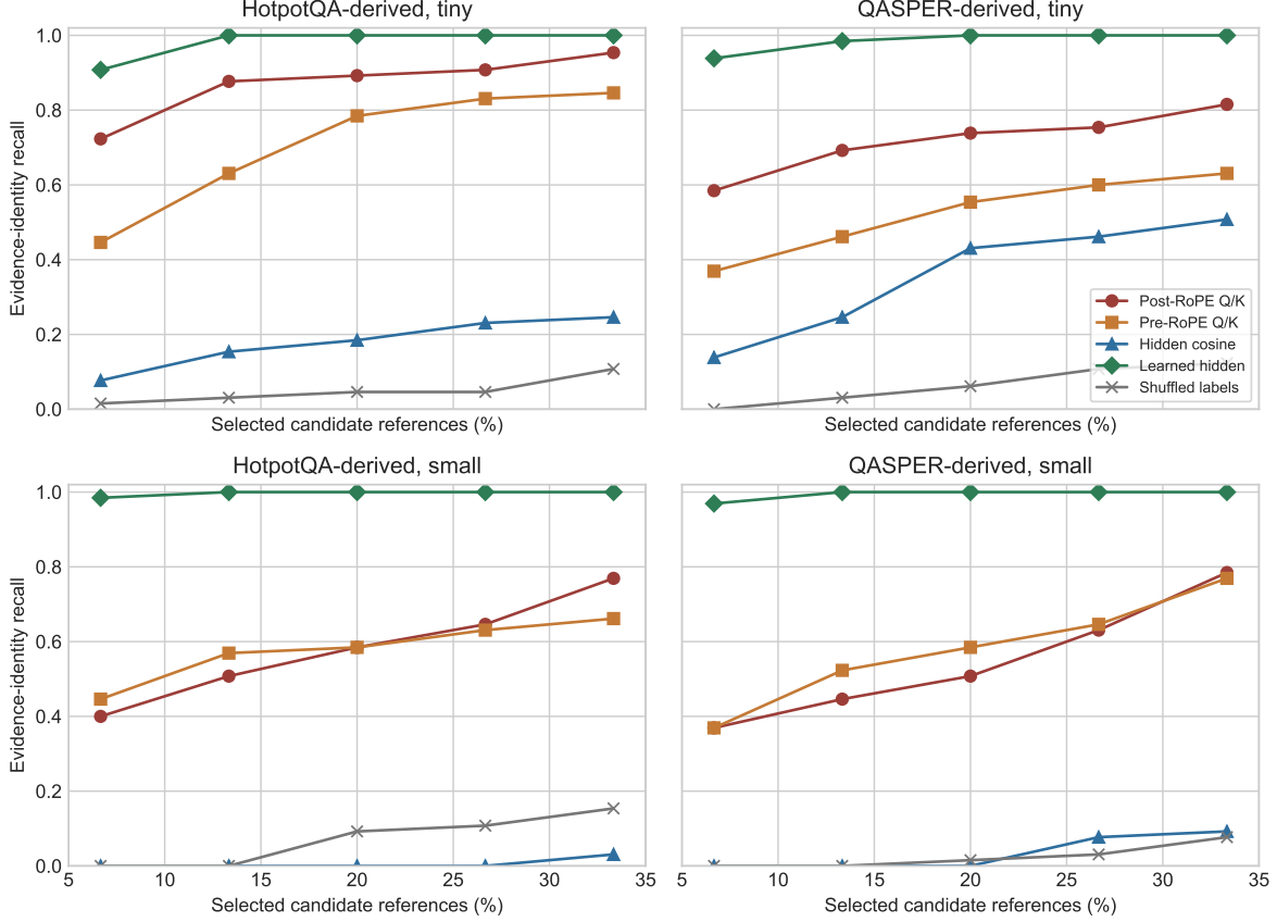
Figure 8: The learned 32-D hidden-state metric dominates raw hidden cosine and the shuffled-label control throughout the sparse range. Post-RoPE and pre-RoPE Q/K remain useful controls but do not define the best evidence-ranking geometry. Curves average five seeds.
