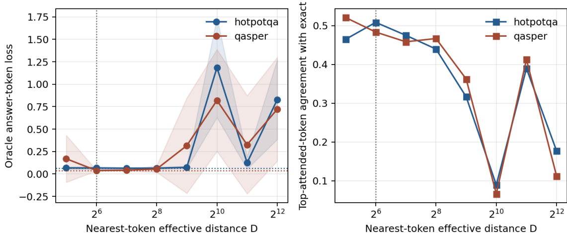
Figure 2: The same retrieved evidence under different RoPE displacements. Dotted horizontal lines show exact-placement loss; the vertical line marks the pooled selected value D = 64 . Bands are one standard deviation over five seeds. Remote placement can sharply damage loss and top-token agreement, but the useful near range has no stable winner.
