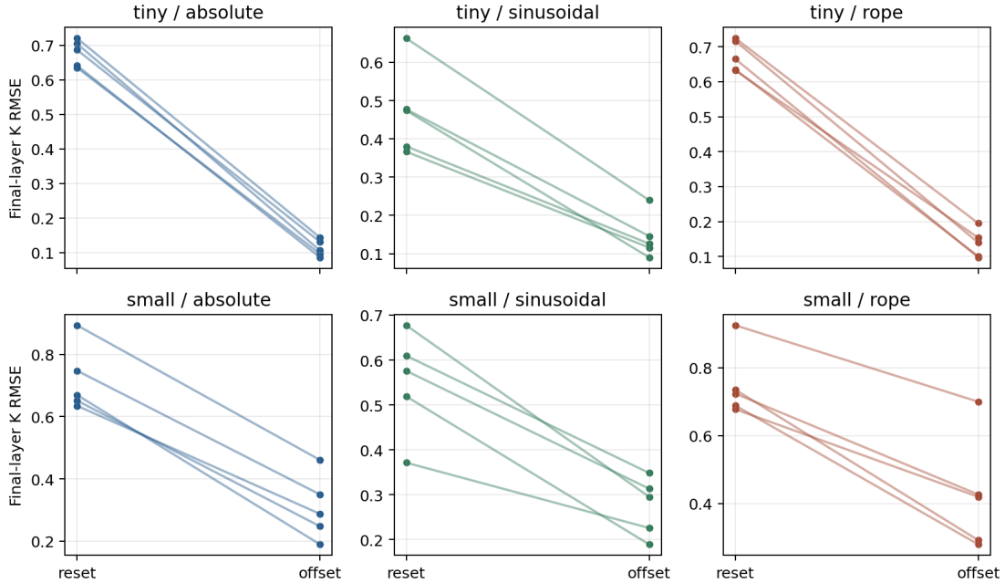
Figure 4: Offsets reduce final-layer K error in all 30 paired runs. The residual after exact layer-0 repair reveals a second problem: missing causal context across encoding blocks.
