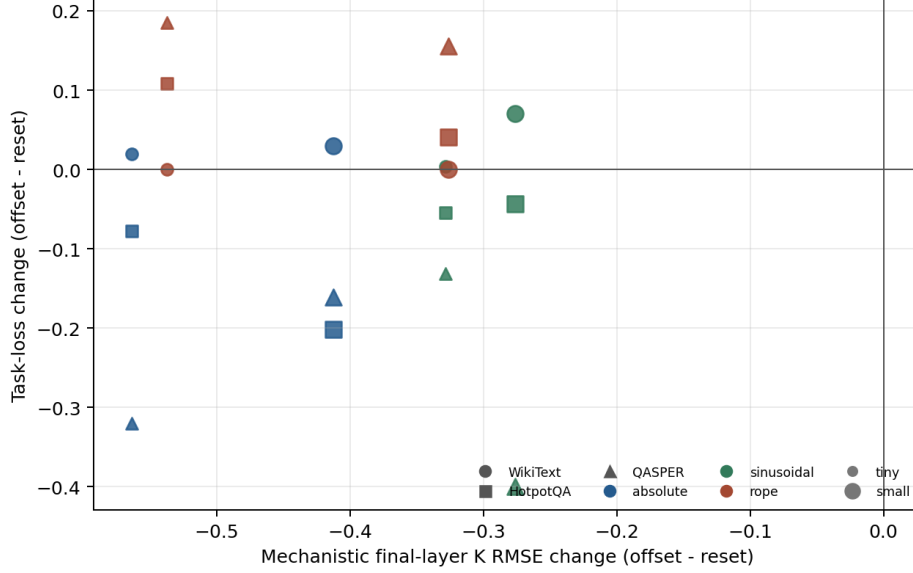
Figure 6: Every point moves left because offsets improve representation fidelity. Task-loss changes cross zero. Correct geometry is therefore not a sufficient predictor of usefulness.
