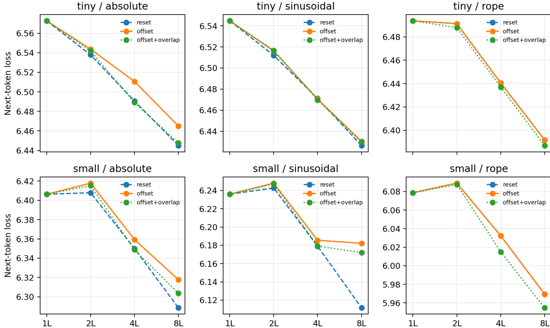
Figure 5: On WikiText-2, offsets sharply improve representation fidelity without a matching loss gain. Overlap gives smaller, more consistent loss changes at almost 1.94\times encoding cost at 8L.
