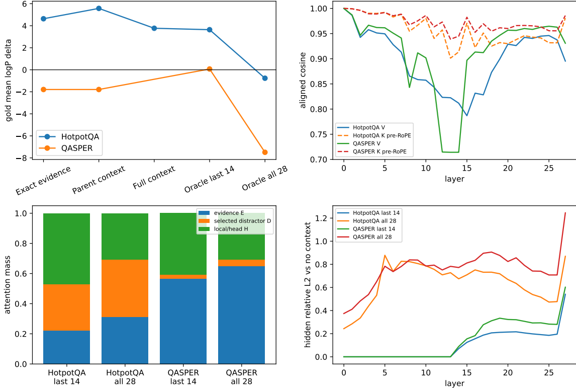
Figure 3: The oracle gap remains after exact discovery and transport. Direct-context controls, aligned K/V similarity, attention support, and residual divergence diagnose distinct stages; no panel alone is presented as a complete causal explanation.
