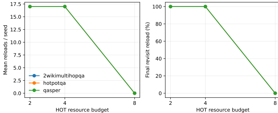
Figure 10: The eight-resource working-set threshold appears consistently across all three datasets.
