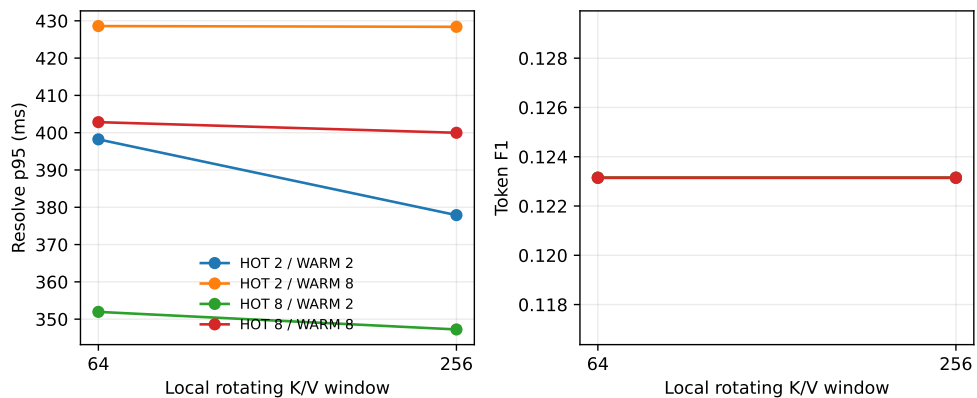
Figure 11: Local-window size has no quality effect in this bounded decode; HOT admission dominates median resolution, while broad WARM retention does not improve the tail on this host.
