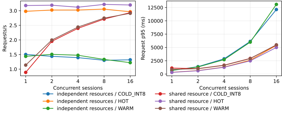
Figure 9: MLX physical-tier concurrency. Shared WARM amortizes one promotion; independent WARM scales storage work with the number of resources.
