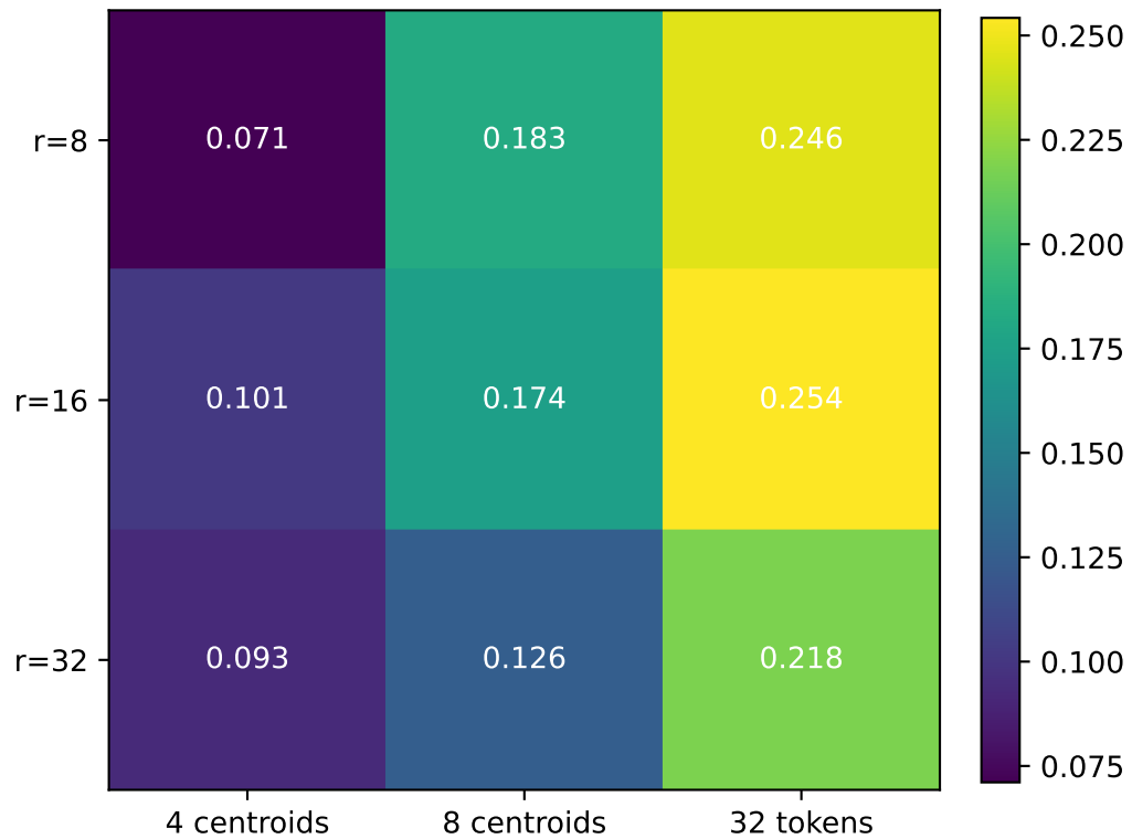
QASPER
