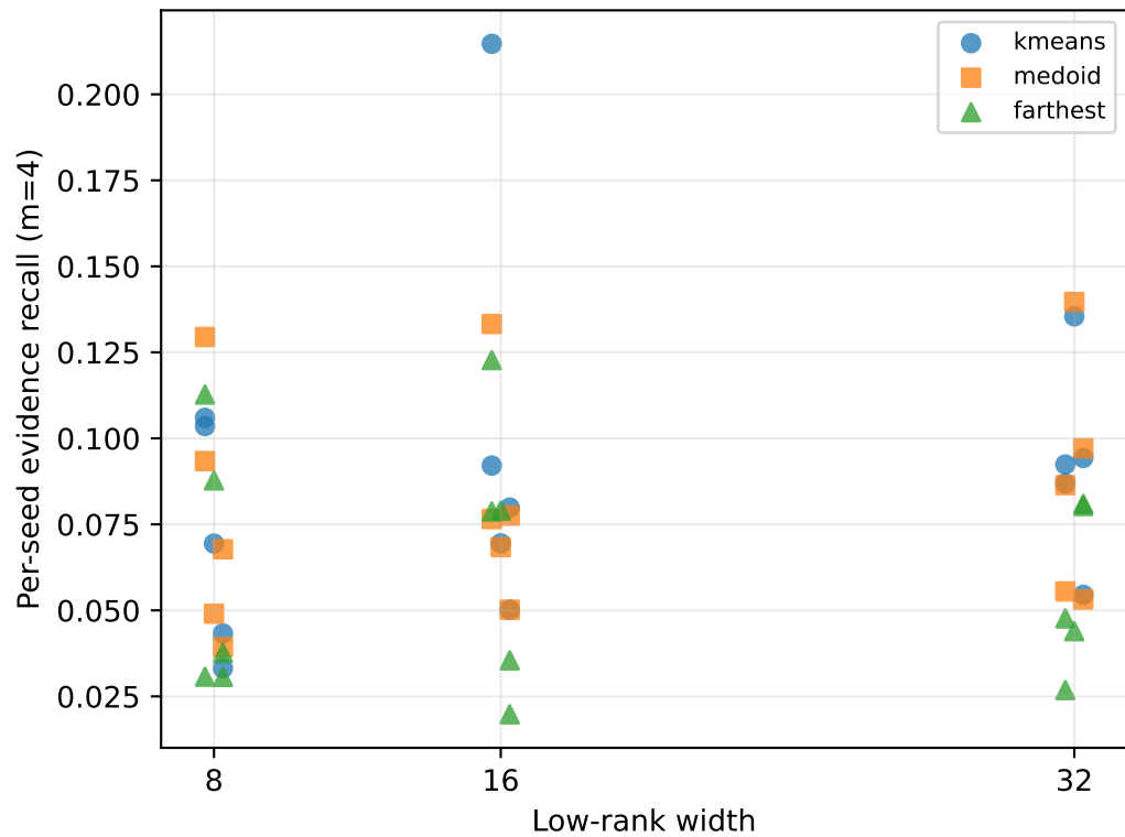
QASPER
