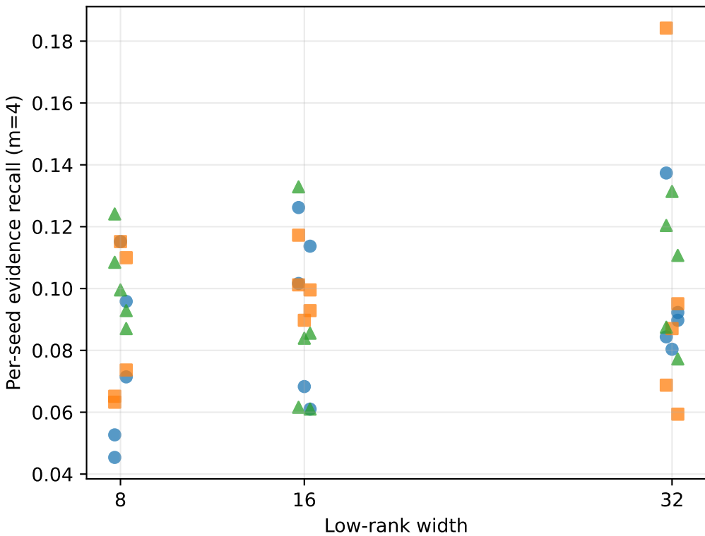
HOTPOTQA
