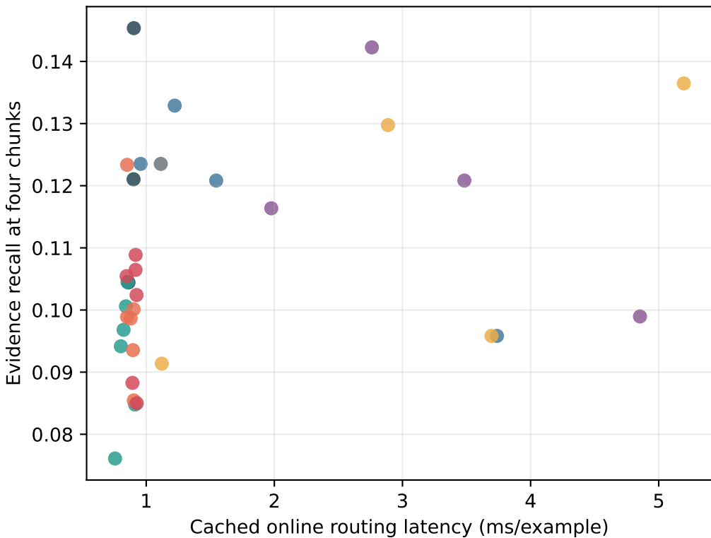
HOTPOTQA
