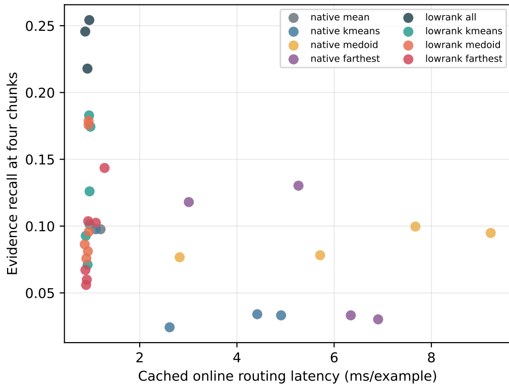
QASPER
