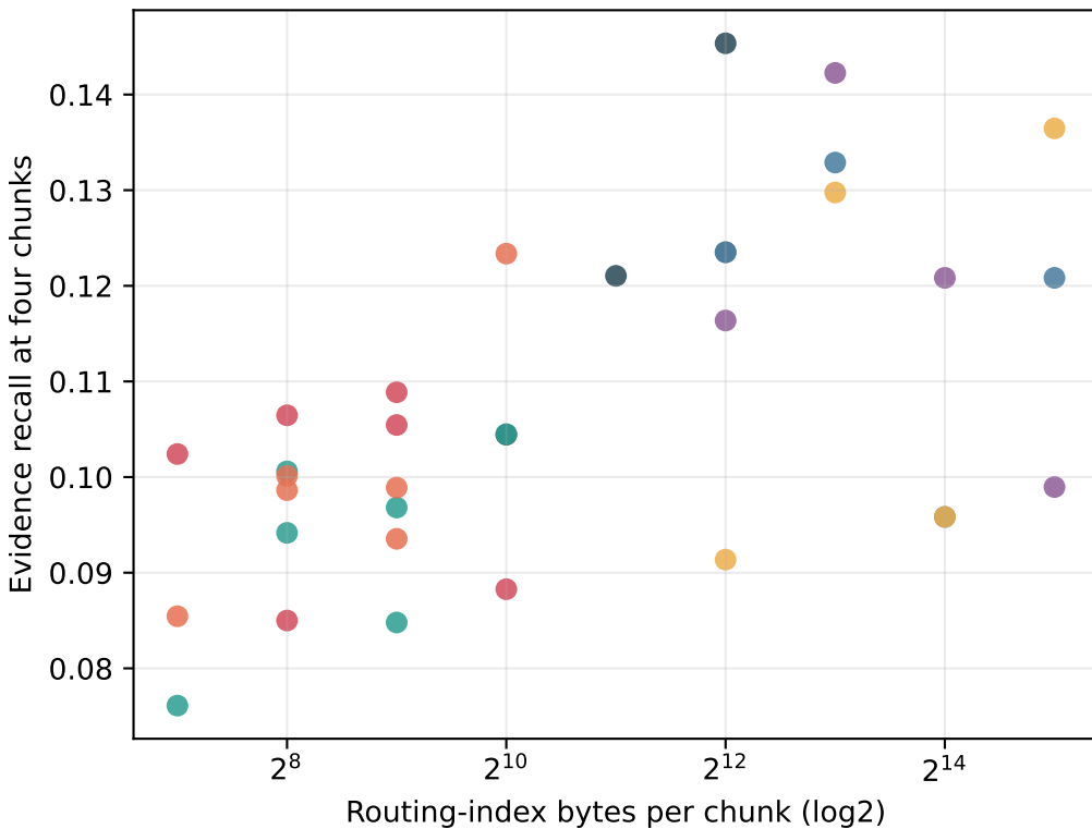
HOTPOTQA
