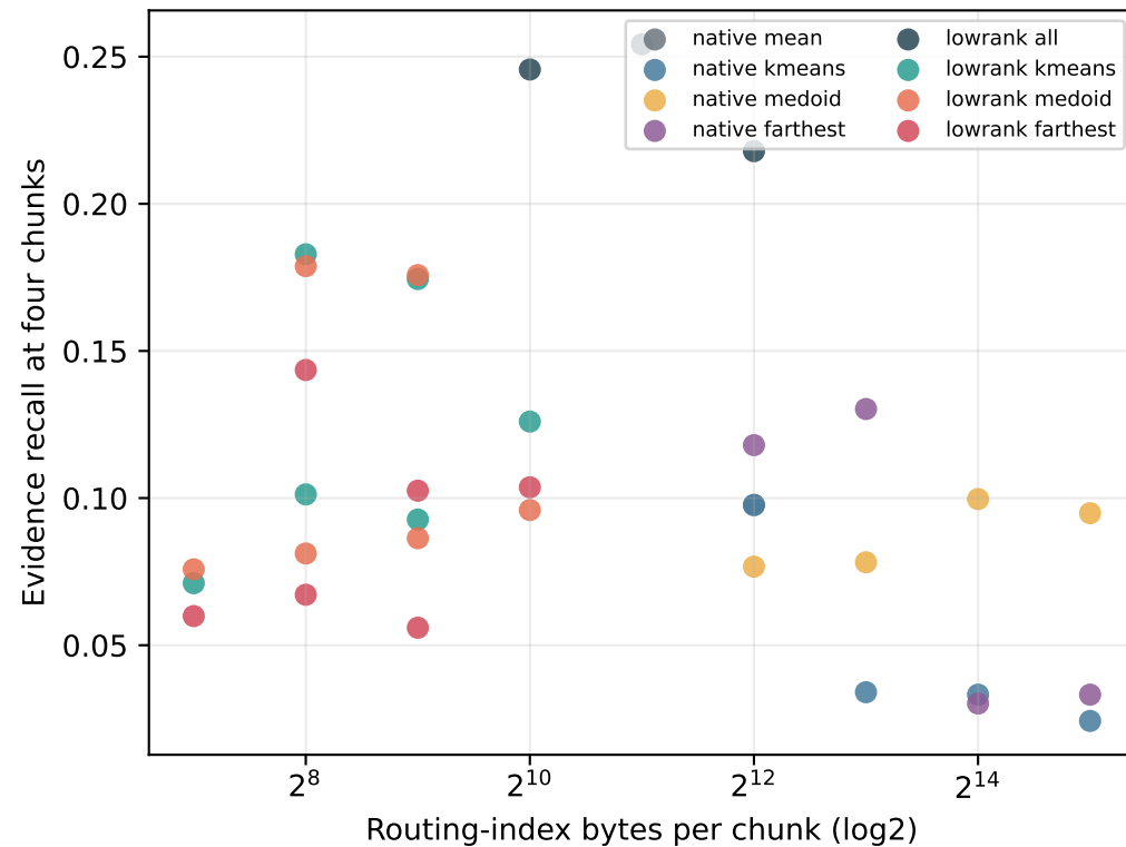
QASPER
