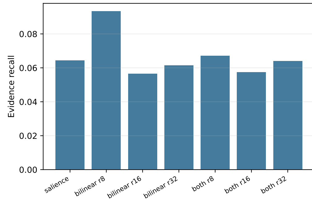
QASPER, m=4
