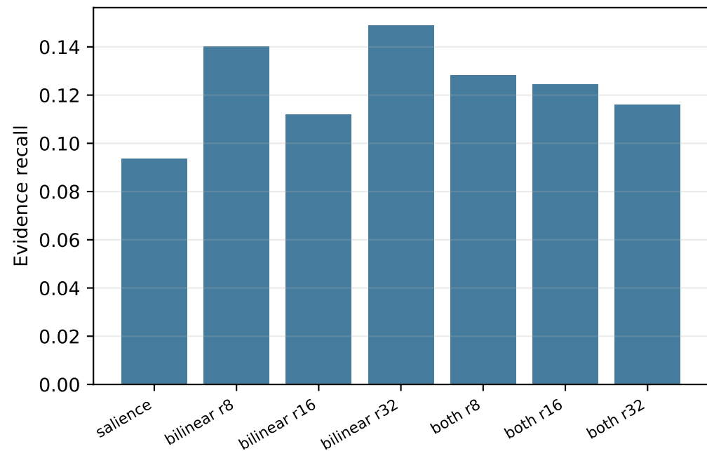
QASPER, m=8
