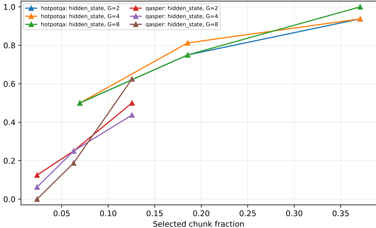
Any-evidence recall
