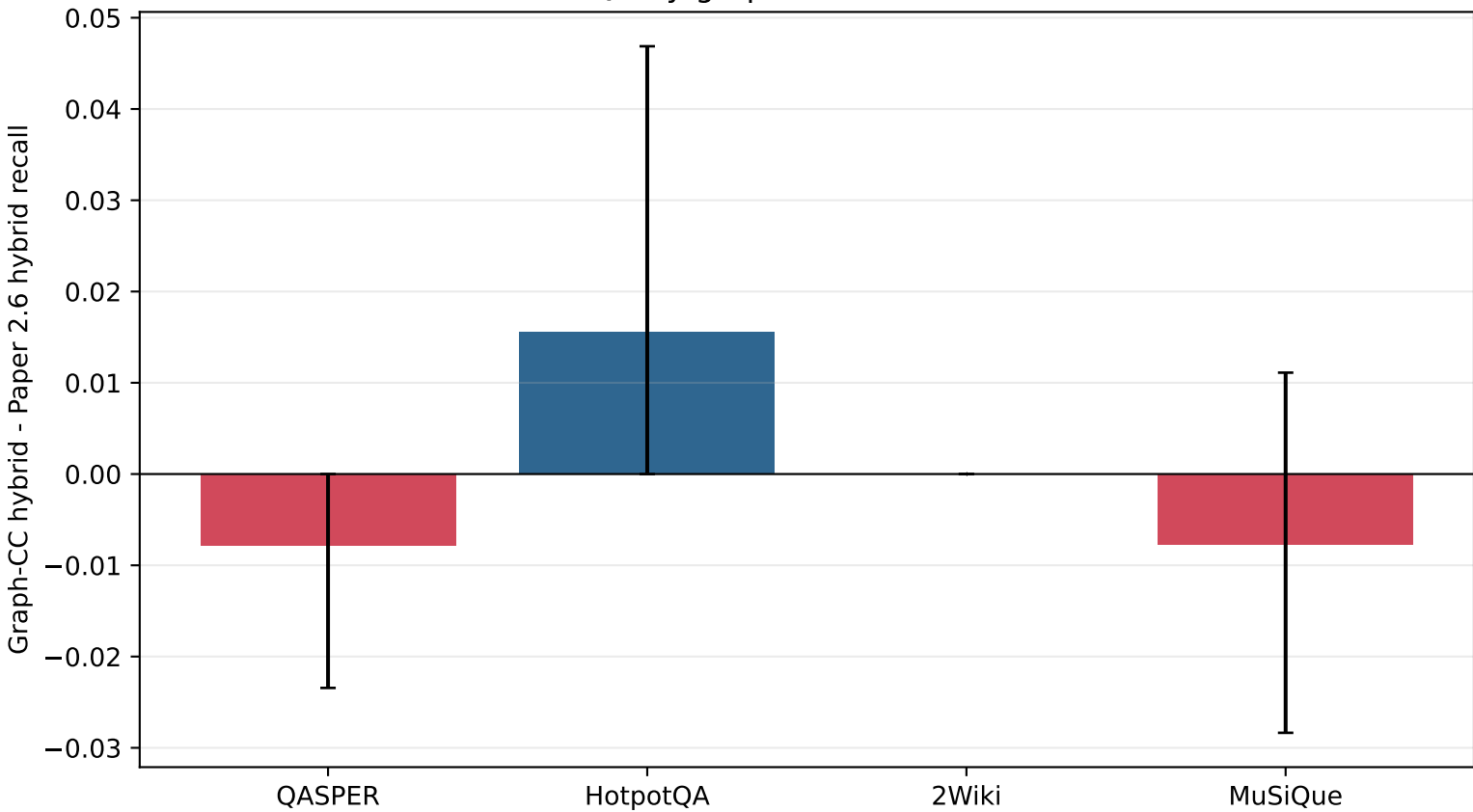
Query-graph retrieval effect
