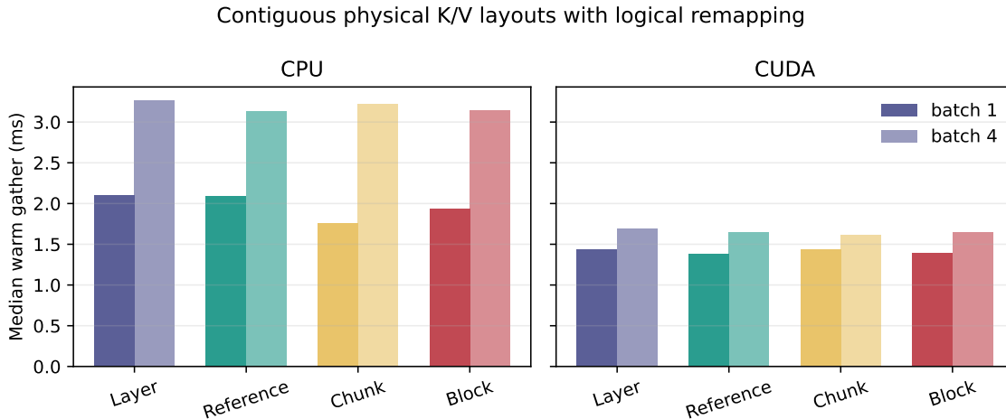
Figure 13: Warm materialization from four physically distinct contiguous stores. Every layout restores the same logical per-layer K/V before attention.
