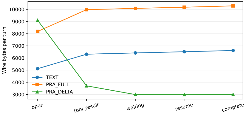
Figure 8: Per-turn JSON bytes for the five-turn task/tool workflow. PRA-FULL preserves explicit metadata but repeats all resource bodies; PRA-DELTA sends a body only for ADD or UPDATE and keeps unchanged resources logical.
