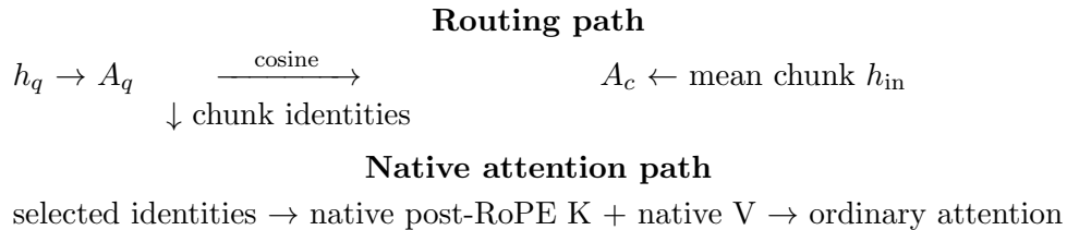
Figure 9: Semantic memory selection and positional attention can use different geometries without changing the selected native K/V payload.
