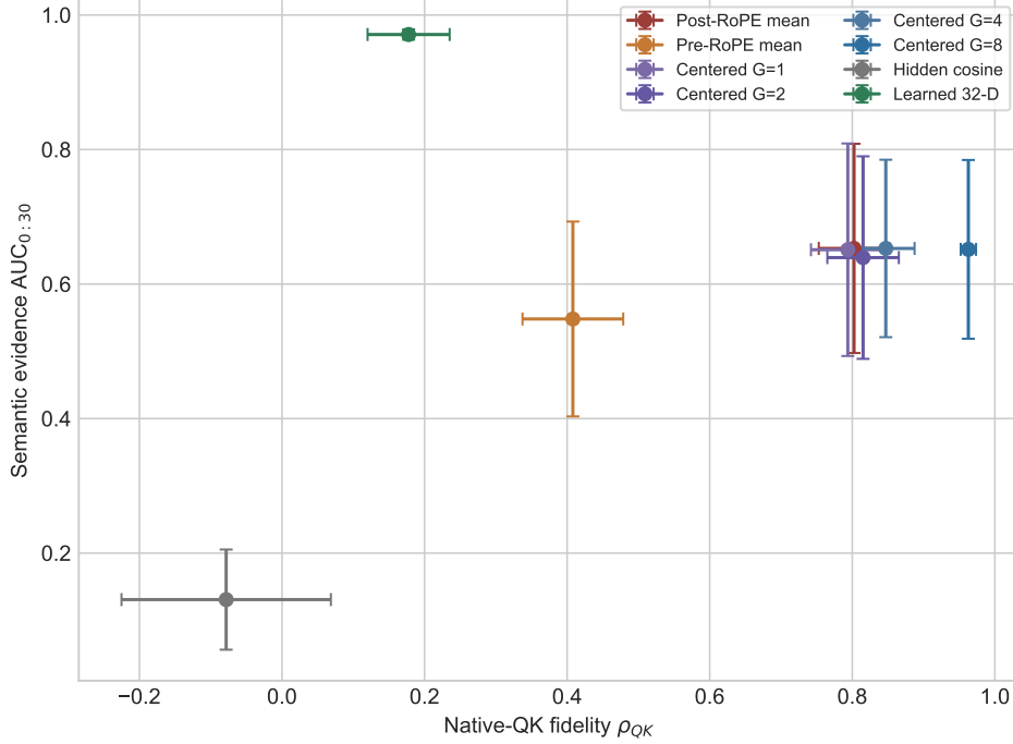
Figure 7: Increasing centered-RoPE resolution closely reproduces native Q/K ranking without improving semantic evidence retrieval; the learned semantic router shows the opposite geometry. Error bars are 95% confidence intervals over five seed-level means.
