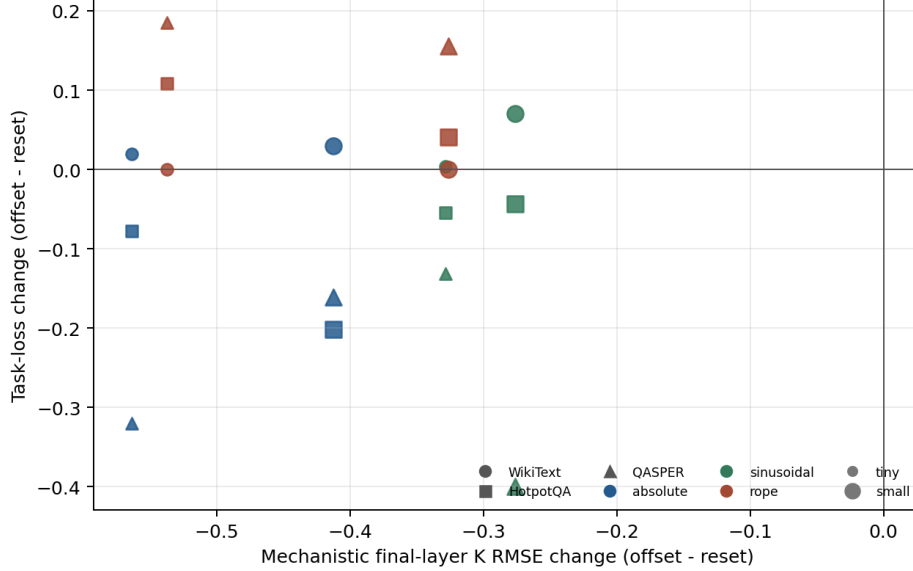
Figure 4: Every point moves left because offsets improve representation fidelity, but task-loss changes cross zero. Correct geometry is not a sufficient predictor of usefulness.
