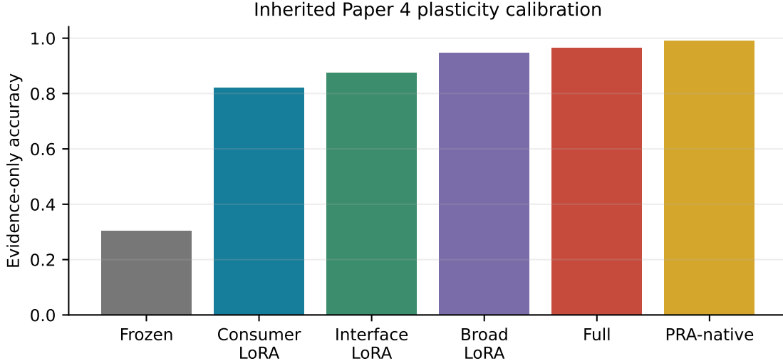
Figure 5: Inherited Paper 4 calibration. Regimes share a controlled oracle-memory task but do not form a model-size scaling curve.
