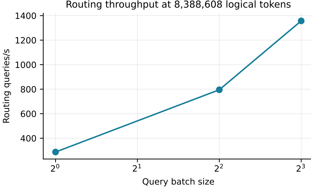
Figure 6: Routing-only exact-search throughput at 8M logical tokens. Batching improves query throughput but does not establish serving throughput or TPOT.
