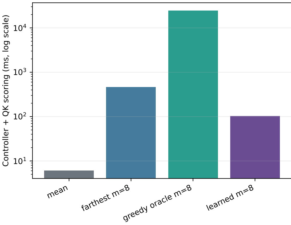
HOTPOTQA
