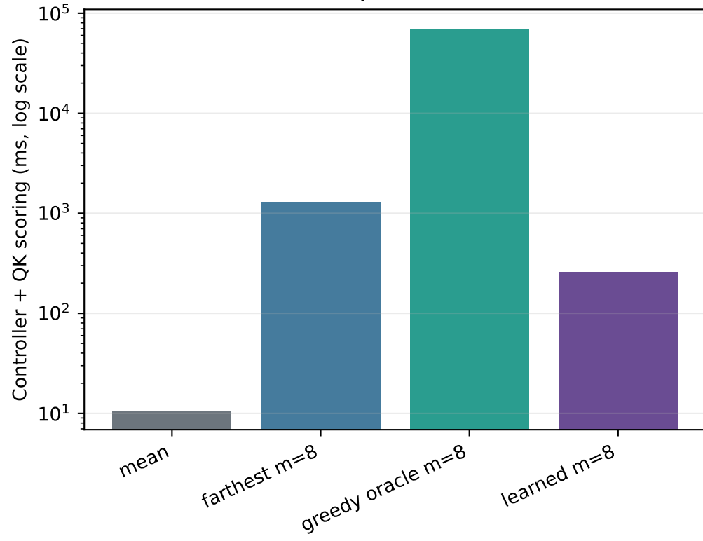
QASPER
