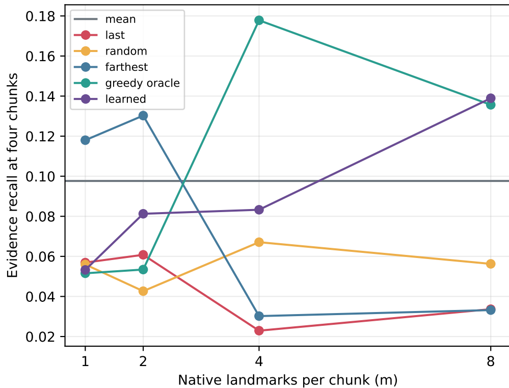
QASPER
