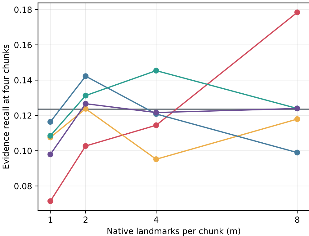
HOTPOTQA
