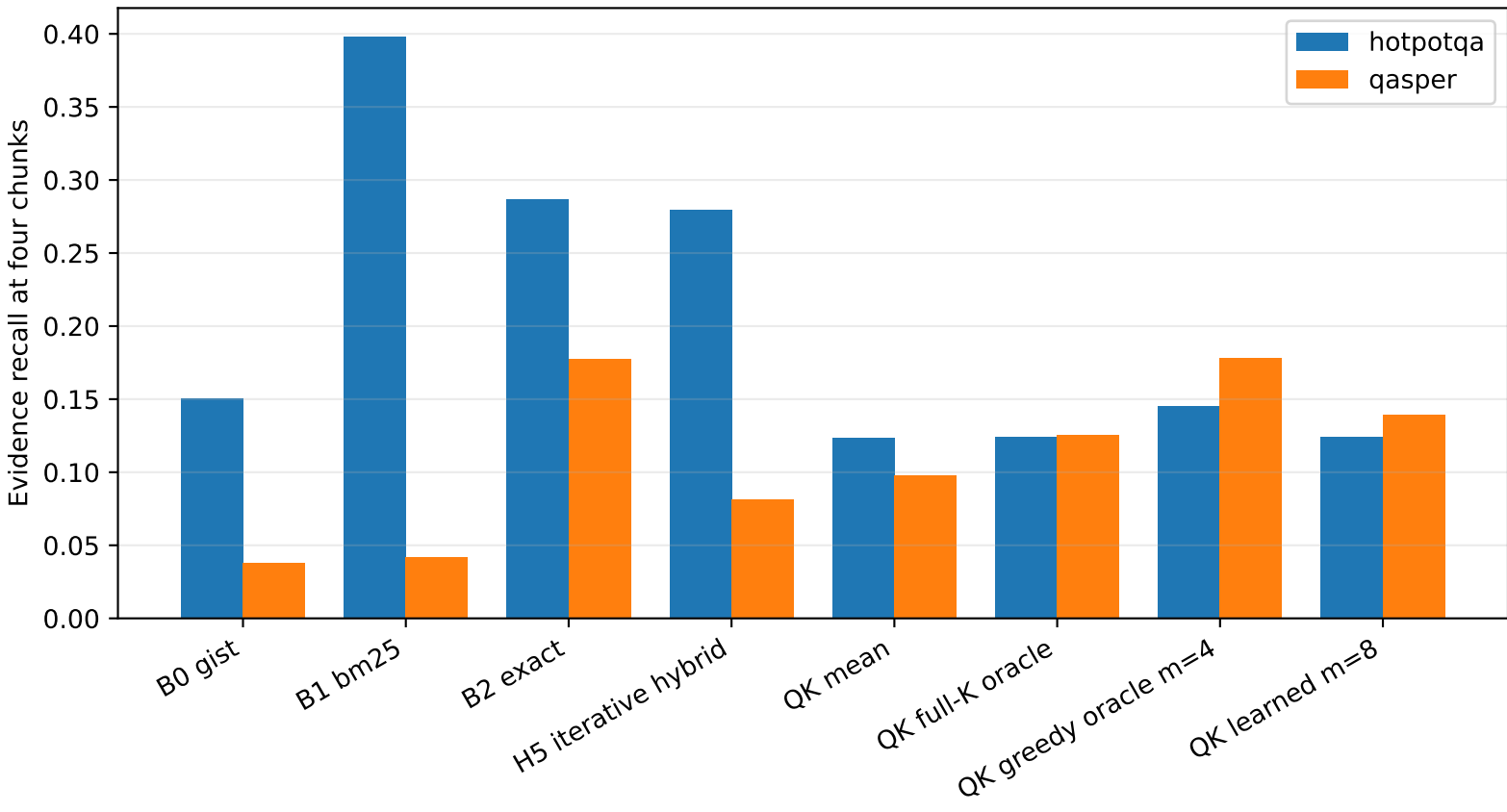
Matched frozen-cohort comparison with Paper 2.6
