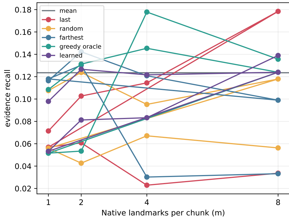
Natural evidence recall
