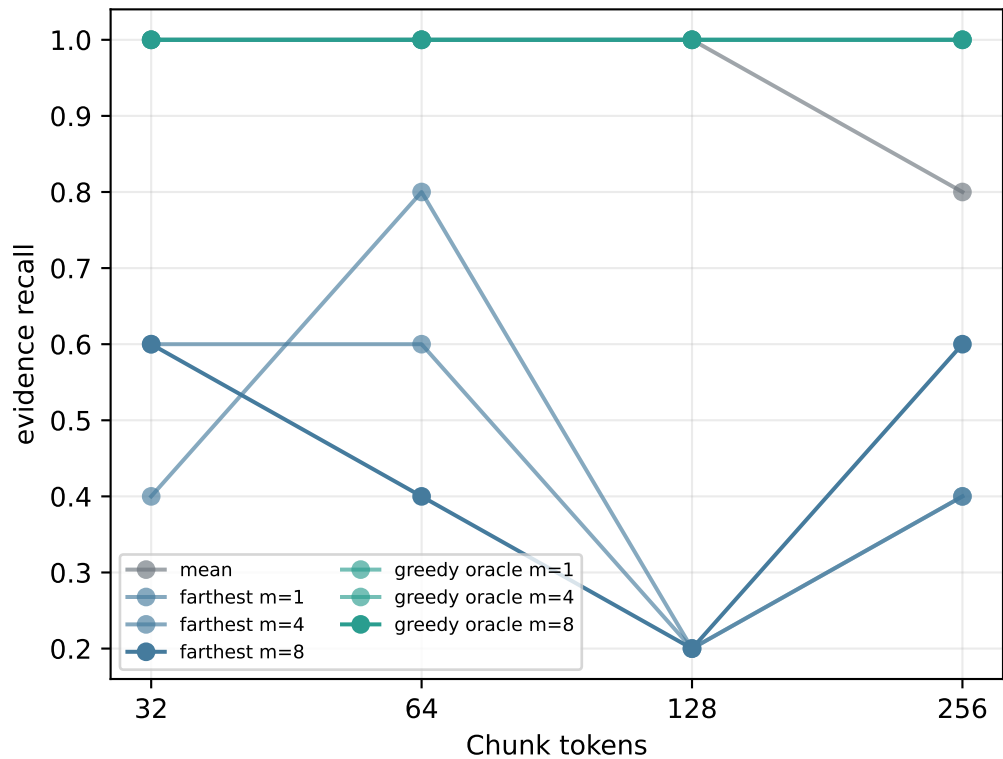
Controlled evidence recall
