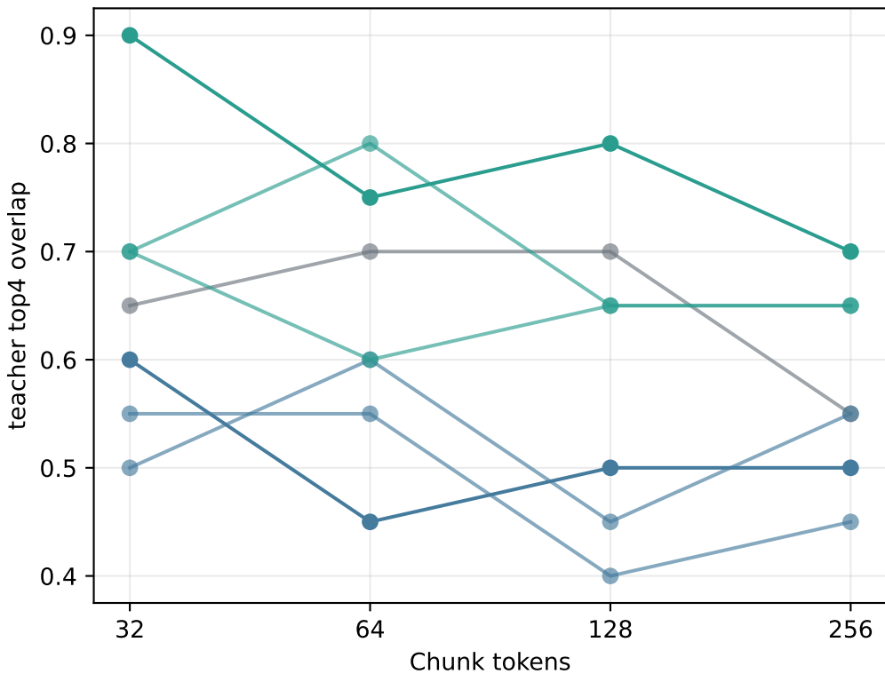
Teacher top-4 preservation
