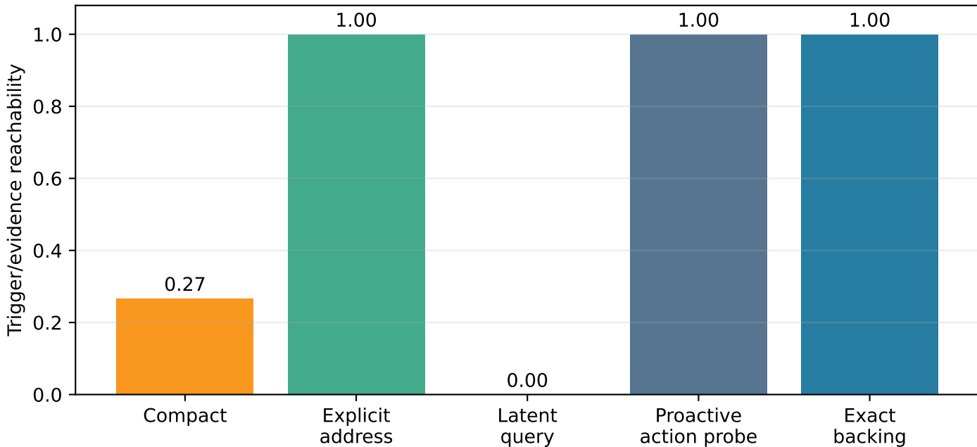
Addressability mechanism check, 45 records
