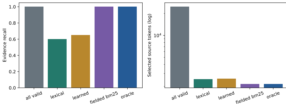
Figure 3: Tracked-source completed-child routing. The all-valid arm preserves recall by materializing the full valid surface. Field-aware local evidence closes the in-cohort oracle gap, but transfer remains unmeasured.
