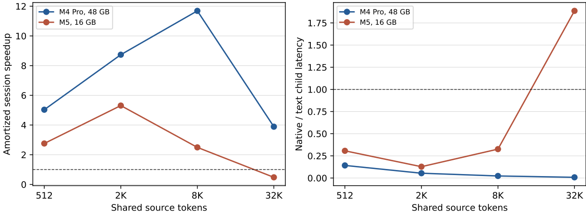
Figure 5: Live MLX reuse across source size and memory-capacity regimes. Left: amortized session speedup at maximum measured fan-out. Right: native/text per-child latency ratio. The dashed line marks parity.
