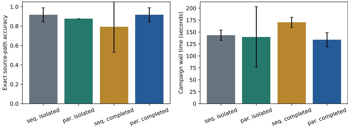
Figure 4: Autonomous accuracy and campaign wall time. Error bars are standard deviations across three seeds; the large isolated-parallel timing variance is part of the result.
