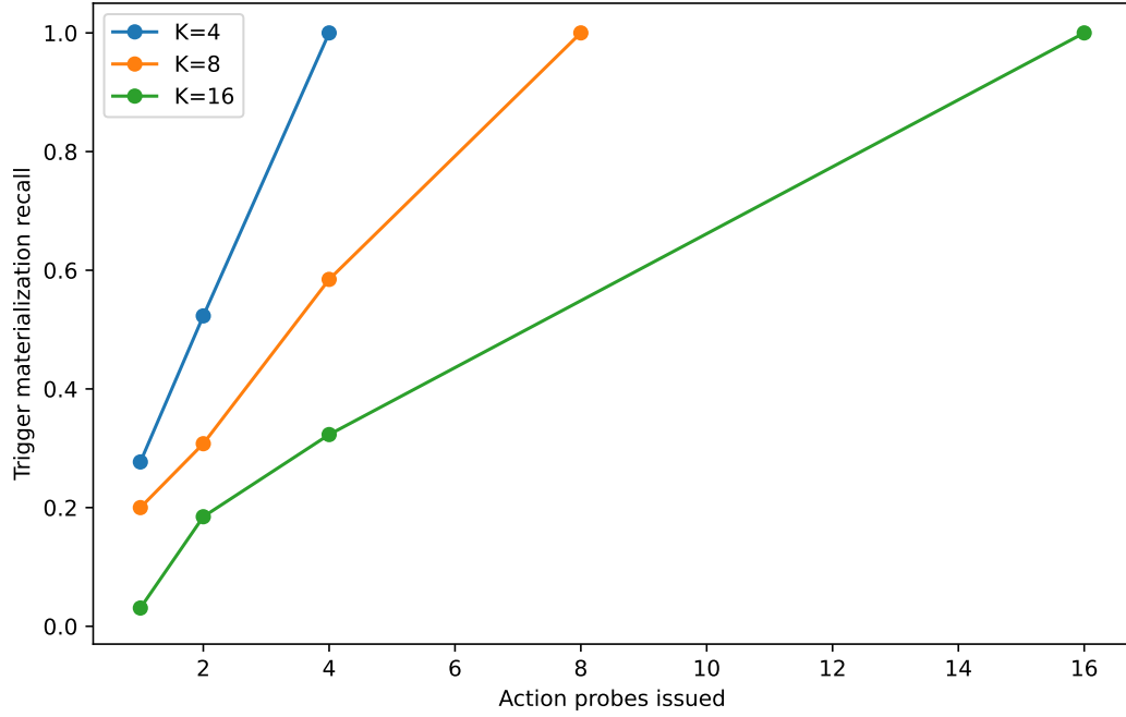
Figure 6: Trigger materialization against probes issued for palettes of K \in \{4, 8, 16\} . Exhaustive action probing is an interpretable upper bound; top- r policies trade hypothesis coverage for fewer expansions.
