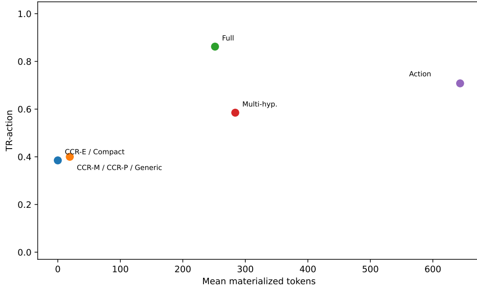
Figure 7: Mean materialized tokens versus latent TR-action. Policies at zero materialization can still exploit compact-view priors; policies farther right pay to expose exact backing evidence.
