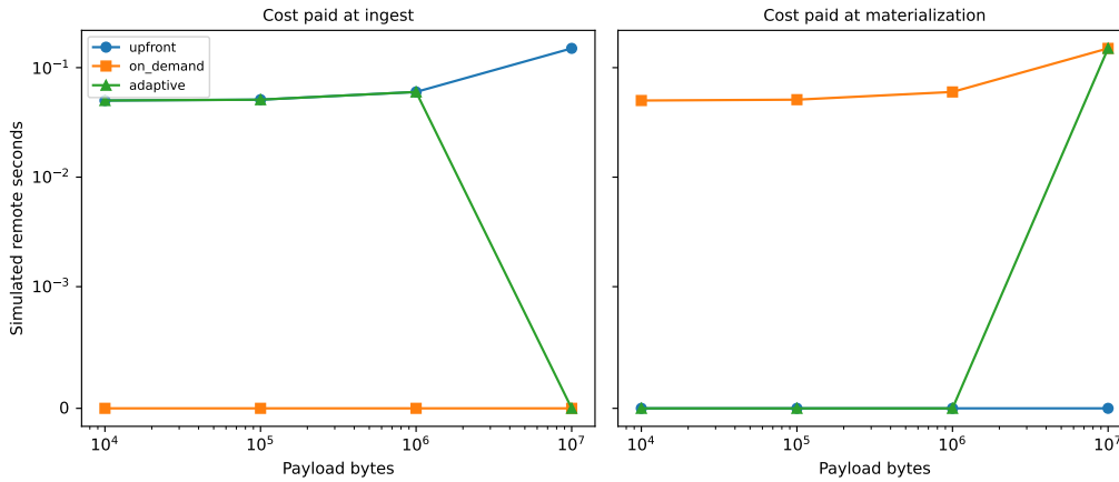
Figure 9: When simulated remote-like transfer cost is paid from 10KB to 10MB. Upfront pays at ingestion, on-demand pays at materialization, and adaptive switches by its declared threshold. RTT and bandwidth components are simulated.
