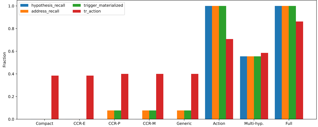
Figure 5: Latent recovery decomposed into hypothesis, address, materialization, and final-action stages. A high later-stage conditional rate cannot compensate for a missing initial hypothesis.
