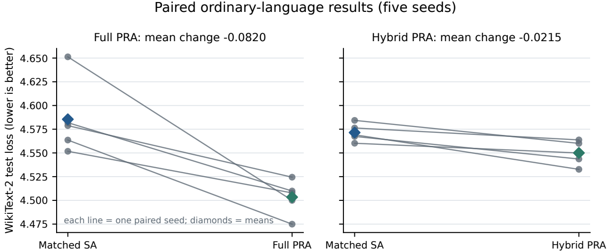
Figure 20: Paired ordinary-language losses for the historical cross-attention-capable backbones. Each line connects one seed to its nearly parameter-matched SelfAttention control; diamonds mark five-seed means. External memory is absent in these runs. The directional result is encouraging but underpowered ( p = 0.0625 ), and it is not a native-KV quality measurement.
