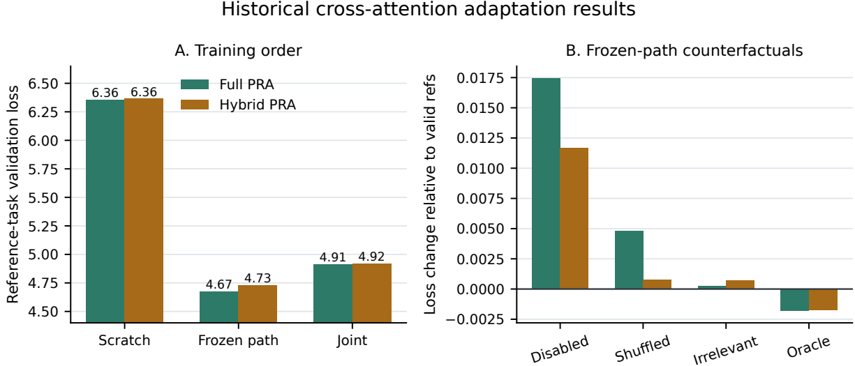
Figure 21: Historical cross-attention adaptation results. Left: frozen-path adaptation finishes substantially below scratch and direct joint tuning for both PRA placements. Right: frozen-path loss changes relative to valid references; positive values are worse. Disabling memory has a visible cost, but shuffled and irrelevant changes and oracle gains are small, so the branch effect is not evidence of content-causal retrieval.
