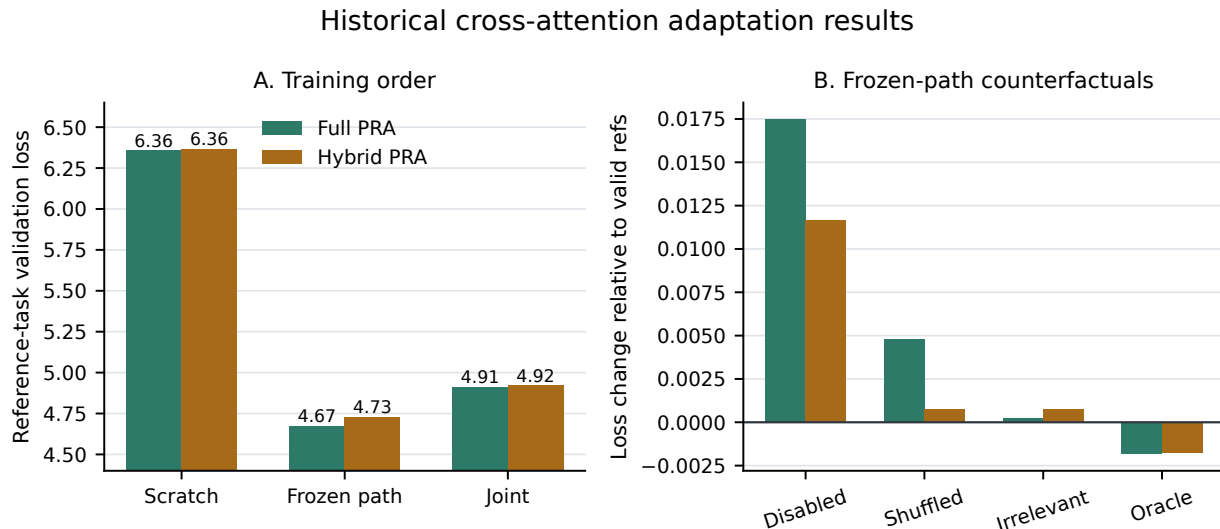
Figure 16: Historical cross-attention adaptation results. Left: frozen-path adaptation finishes substantially below scratch and direct joint tuning for both PRA placements. Right: frozen-path loss changes relative to valid references; positive values are worse. Disabling memory has a visible cost, but shuffled and irrelevant changes and oracle gains are small, so the branch effect is not evidence of content-causal retrieval.
