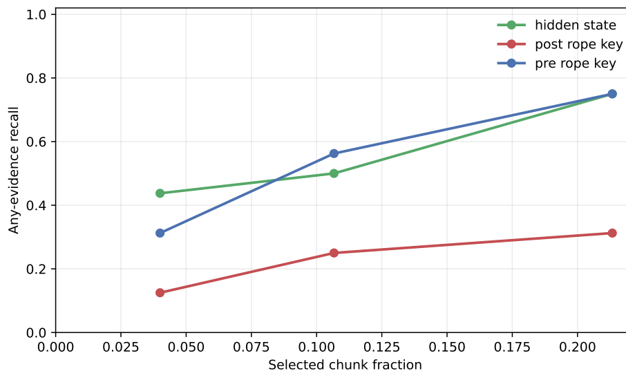
Figure 9: Qwen parameter-free routing diagnostics. Semantic hidden-state and pre-RoPE summaries dominate the post-RoPE key mean for evidence selection, while every fixed selected identity still materializes the same native post-RoPE K/V. This 16-example transfer control is smaller than the learned-router cohort and is not a paired leaderboard with it.
