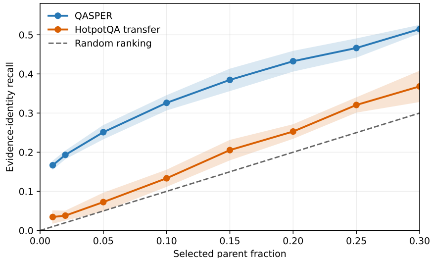
Figure 8: Gemma routing quality is sparse-budget and domain dependent. Five-seed evidence-identity recall is useful on QASPER, its training domain, and transfers more weakly to HotpotQA. Neither curve reaches 0.80 before exhaustive selection.
