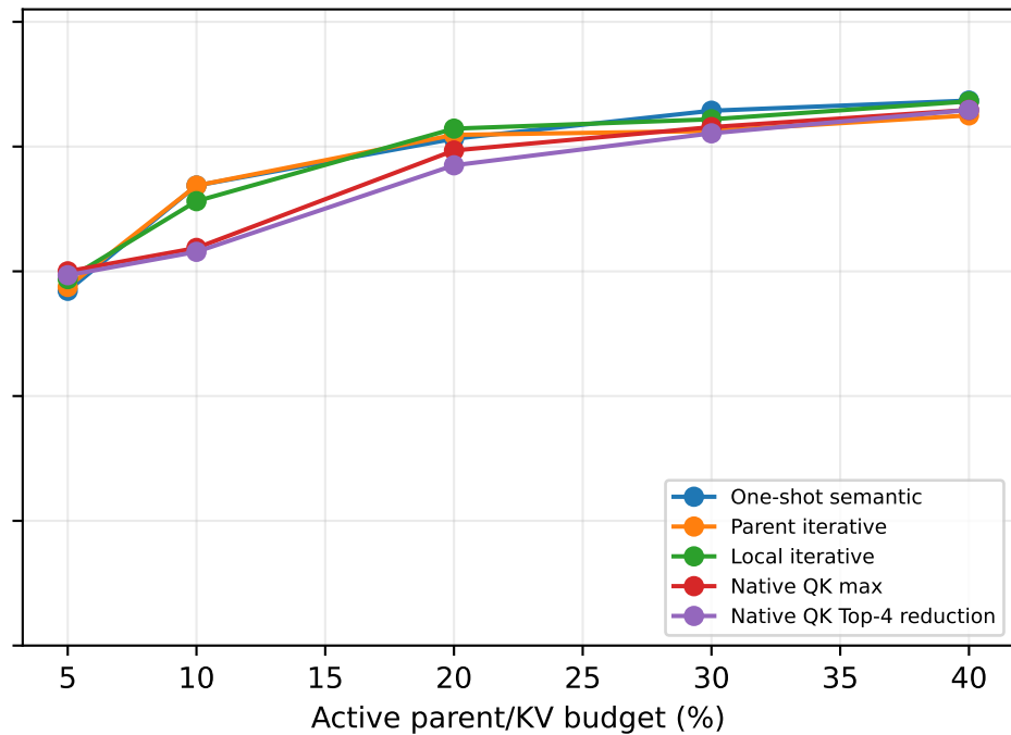
qasper
