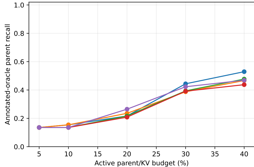
hotpotqa
