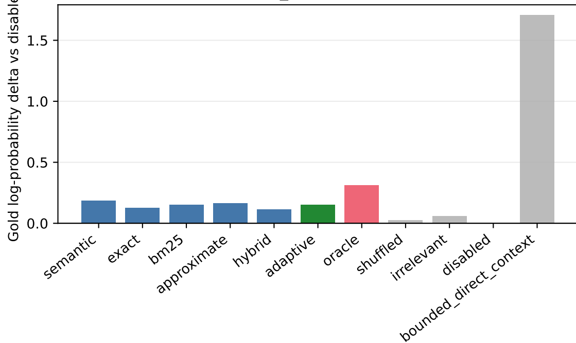
smollm2_135m / hotpotqa
