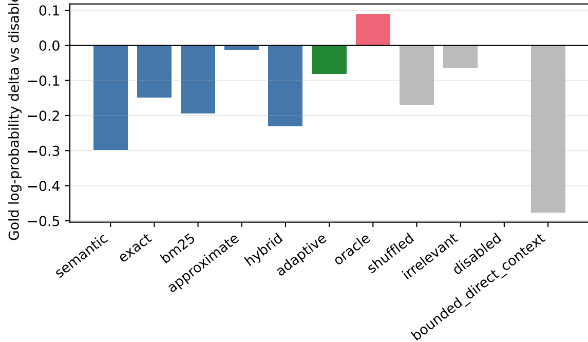
qwen3_0_6b / qasper
