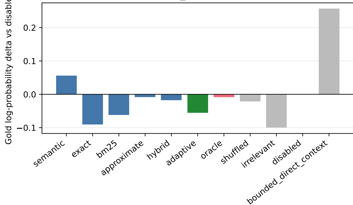
smollm2_135m / qasper
