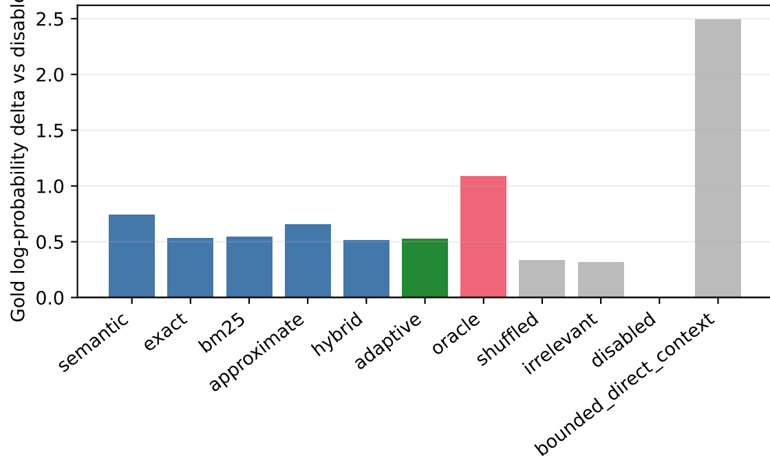
qwen3_0_6b / hotpotqa
