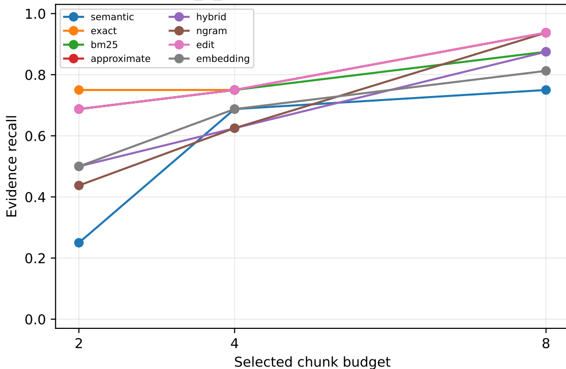
smollm2_135m / hotpotqa (32-token chunks)
