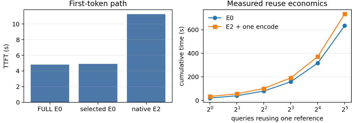
Figure 3: Left: measured first-token cost. Right: cumulative measured request time when one reference is reused. E2 has no finite latency break-even in the current trace because its warm per-query slope remains above E0 even before adding the one-time 10.88-s reference encoding cost.
