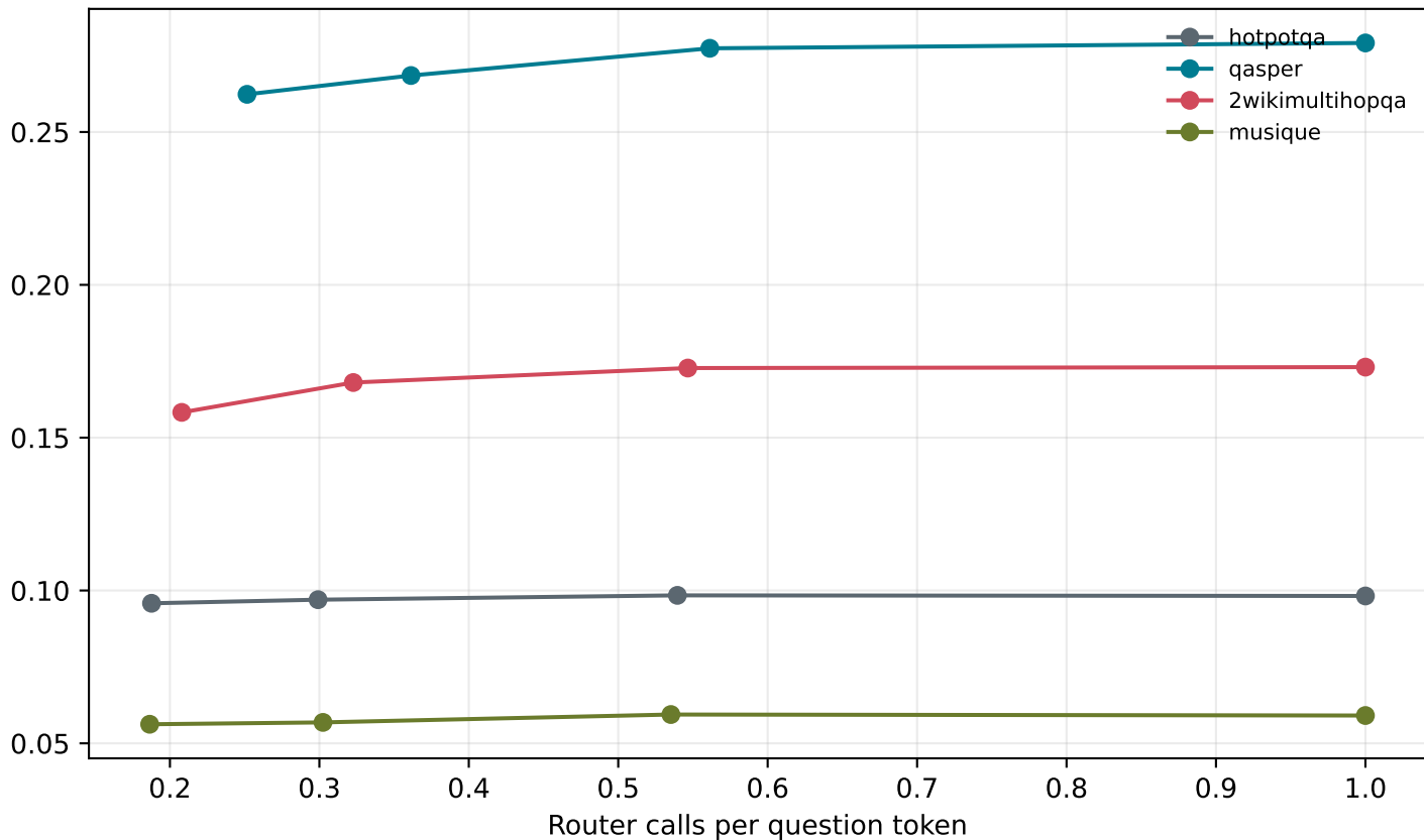
Trajectory evidence recall @ 4
