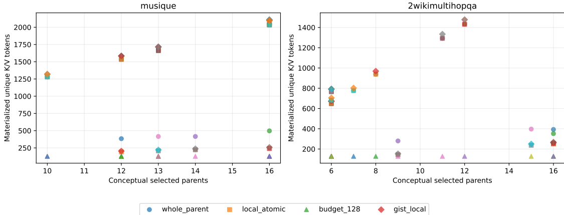
Figure 14: Conceptual parent count versus physical K/V. Fixed budgets decouple the axes, but quality depends on whether the budget preserves all required evidence regions.
