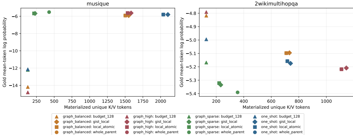
Figure 13: Frozen selection-by-materialization factorial. The same conceptual selection can occupy different physical K/V points; broad selected spans sometimes leave no local compression room.
