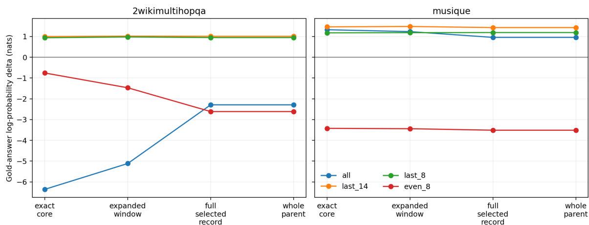
Figure 11: Materialization geometry crossed with consumer placement. The late contiguous bands are robust; all-layer and evenly spaced consumption expose workload-specific interference.
