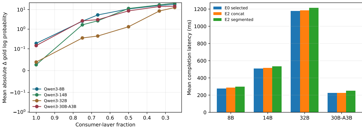
Figure 12: Left: consumer-depth sensitivity across model scale. Right: the selected-text, concatenated-native, and segmented-native execution costs on the M4 Pro. The figure calibrates placement; it is not a materialization-width or serving-throughput result.
