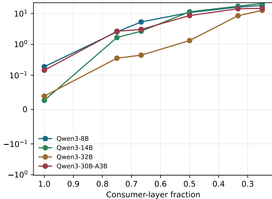
Mean absolute \Delta gold log probability
