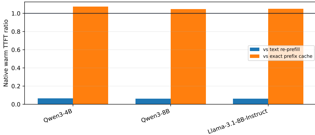
Figure 12: Warm native TTFT relative to text re-prefill and exact-prefix reuse. The horizontal line marks equal cost; lower is better.
