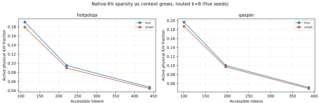
Figure 3: Fixed k = 8 keeps physical selected K/V nearly flat as candidate memory grows. The resulting active fraction falls to 4.4–4.9% at 256 addressable units.
