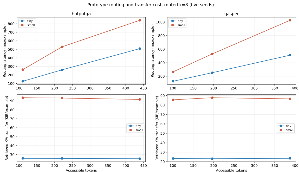
Figure 14: Prototype routing and transfer cost. Fixed- k K/V transfer remains nearly constant, while exhaustive candidate scoring dominates end-to-end execution.
