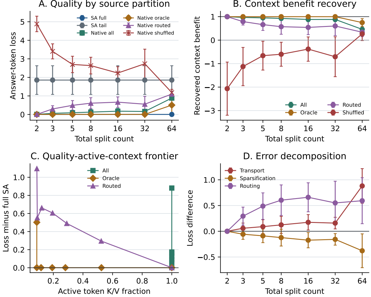
Figure 11: QASPER-derived replication over five paired seeds. Sparse oracle K/V preserves dense-context benefit through split 32, while all-memory composition, routed selection, and 64-way fragmentation remain limiting.
