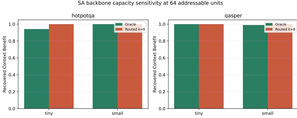
Figure 13: Backbone capacity at 64 units. The small tier improves annotated-oracle robustness and maintains routed quality, but also increases model and K/V width.
