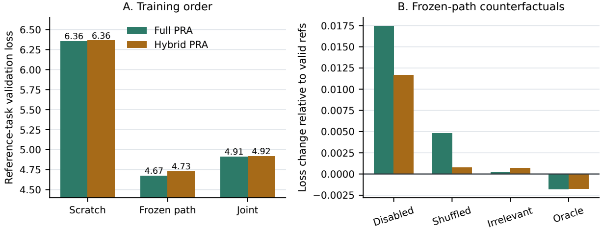
Figure 16: Historical cross-attention adaptation results. Left: frozen-path adaptation finishes substantially below scratch and direct joint tuning for both PRA placements. Right: frozen-path loss changes relative to valid references; positive values are worse. Disabling memory has a visible cost, but shuffled and irrelevant changes and oracle gains are small, so the branch effect is not evidence of content-causal retrieval.
