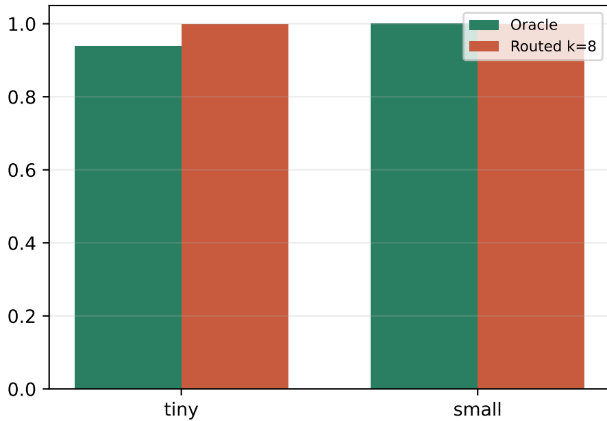
hotpotqa
