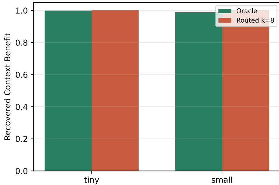
qasper
