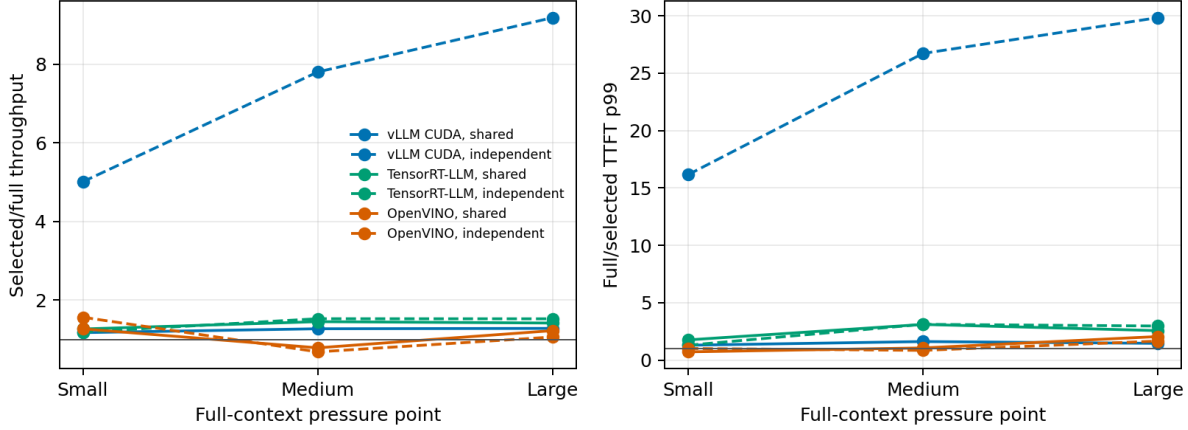
Figure 22: Within-engine throughput and TTFT-tail ratios over three context pressure points. Absolute rates are not compared across dissimilar hardware.
