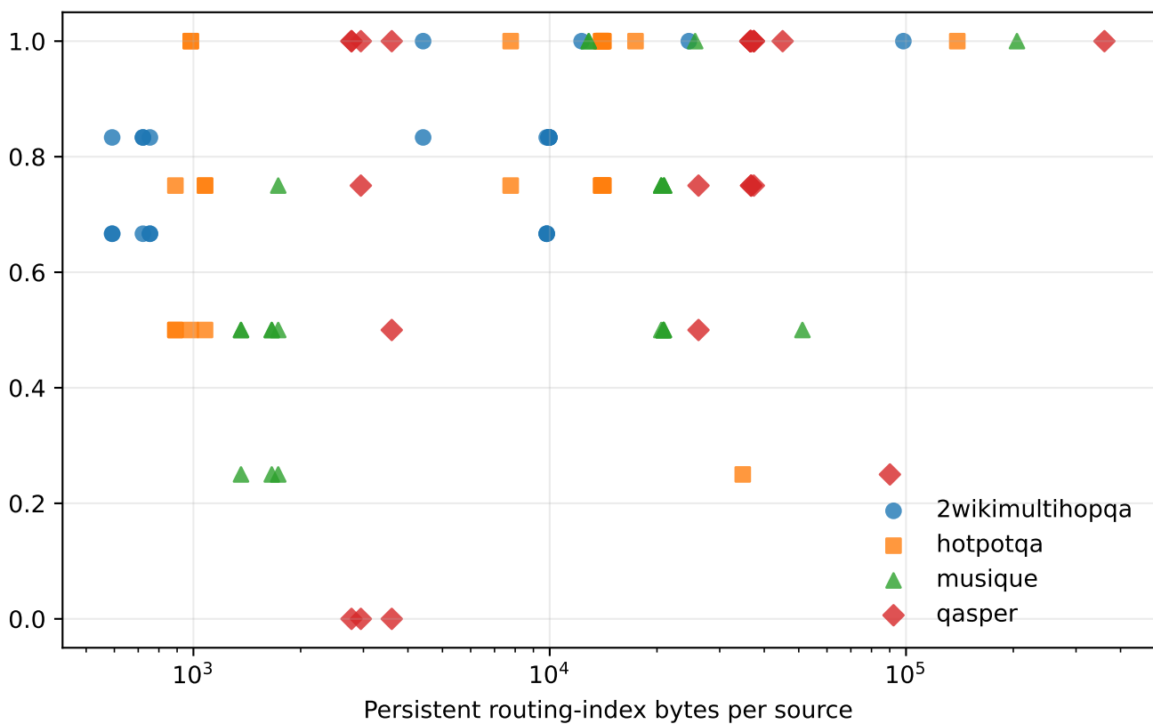
Evidence recall @ 4
