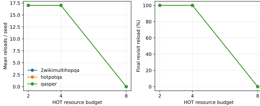
Figure 25: Sustained pressure exposes a working-set threshold rather than a quality effect: once all eight resources fit, reloads disappear.
