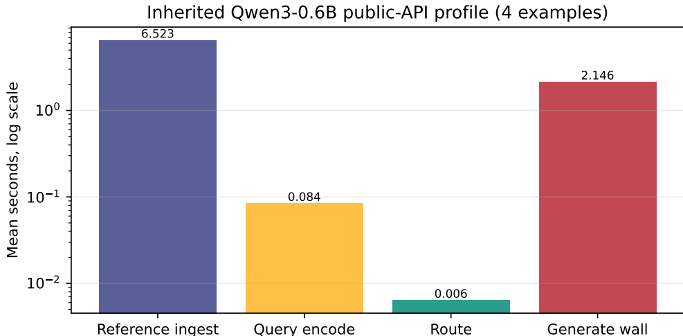
Figure 17: Inherited Paper 2 Qwen3-0.6B profile over four examples. The log scale shows that routing time is small relative to native reference encoding and generation on that protocol.
