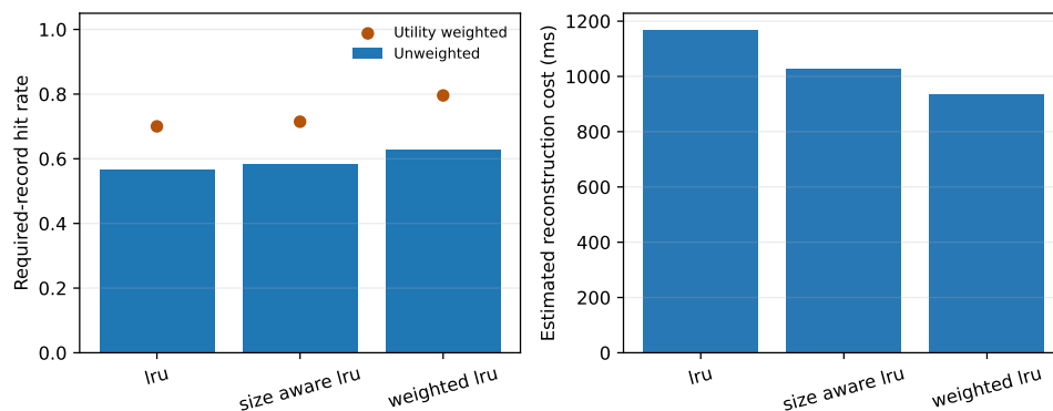
Figure 19: Equal-quota retention on a mixed task, document, and tool-result trace. Weighted policy protects active task state and shared documents while allowing reconstructable transient records to churn.
