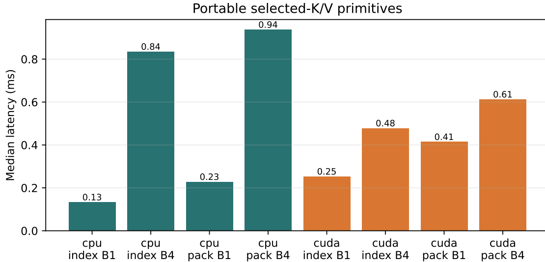
Figure 14: Portable primitive latency. This older GPU does not make small batch-one gathers faster than the CPU, but CUDA scales better at batch four.
