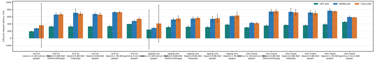
Figure 22: HOT, WARM, and COLD request p50 with p95–p50 upper whiskers. WARM recovery is reliable, but synchronous promotion remains visibly expensive.
