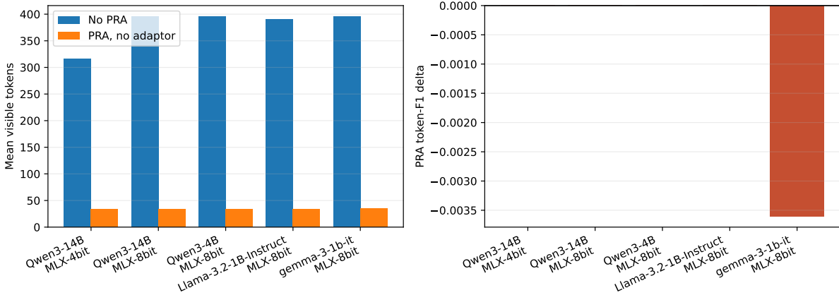
Figure 30: Observed visible-context accounting and generic-PRA token-F1 change by exact precision encoding. The plot deliberately excludes planned rows; absence is not rendered as zero.
