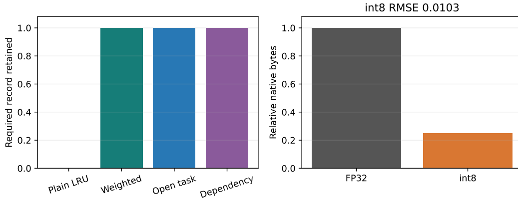
Figure 20: Engine-neutral retention controls and generic symmetric-int8 byte transport. The int8 result is a codec diagnostic; model-specific quality and active-attention bytes remain separate gates.
