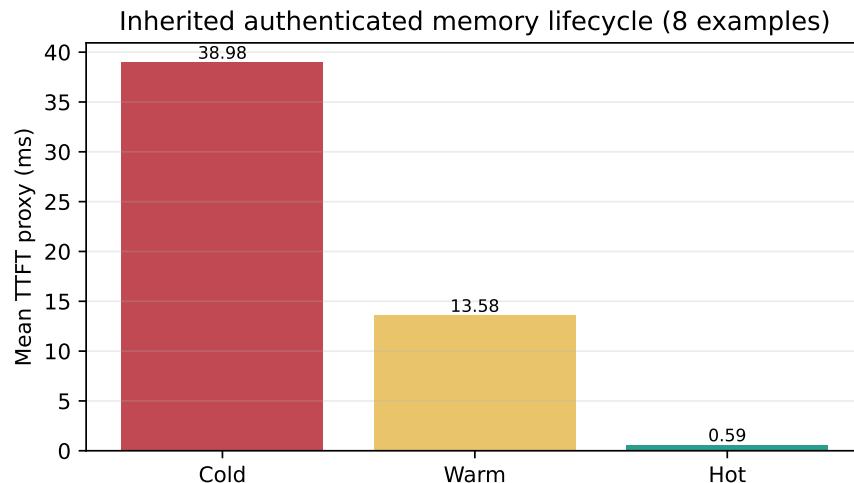
Figure 18: Inherited Paper 4 lifecycle proxy over eight examples. Cold includes fetch and native encoding; warm reuses native encoding; hot reuses selected K/V.
