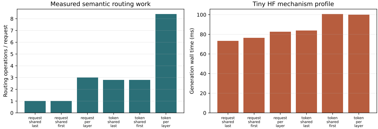
Figure 13: Five-seed tiny-HF mechanism profile. Routing operations validate the execution contract; wall time is host- and model-specific and is not a serving speed claim.
