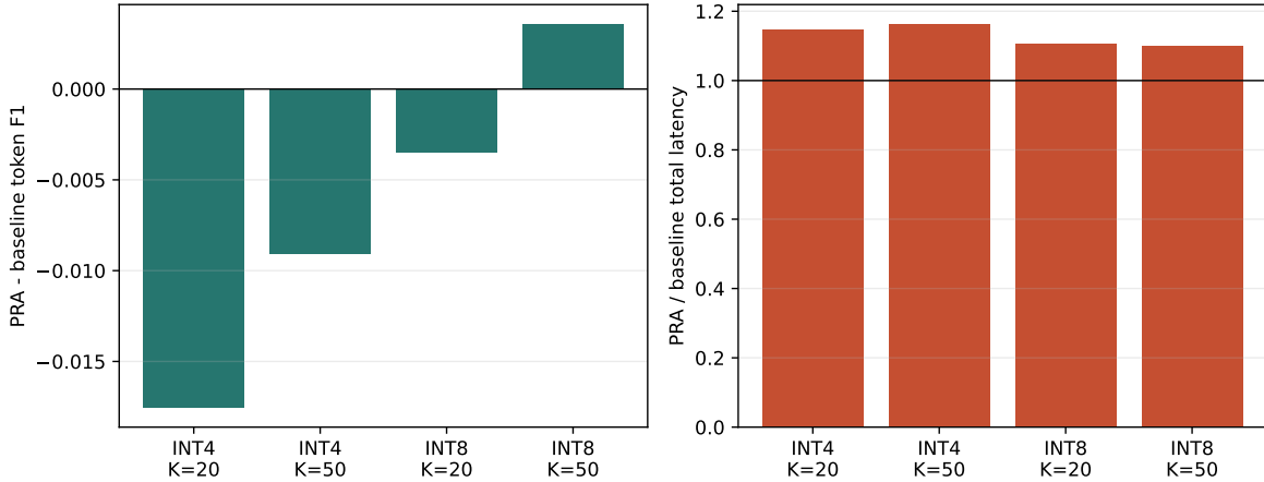
Figure 31: Quality and latency changes for the matched INT4 and INT8 deployed pipelines. The small one-seed cohort is directional evidence, not a precision invariance claim.
