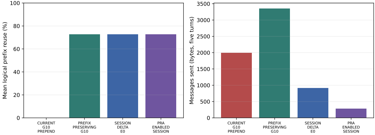
Figure 10: Five-turn deterministic gateway profile. The left panel reports logical reuse of the exact prior serialized message prefix after turn one; the right reports message bytes sent. Resource bytes are reported separately in Table 12.
