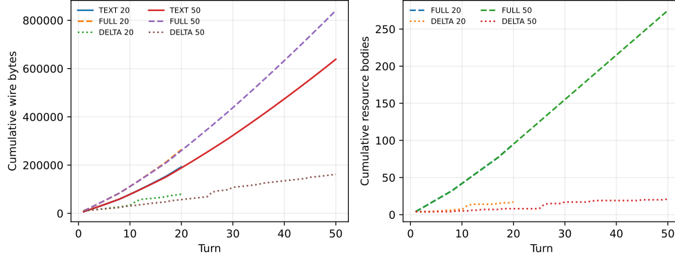
Figure 12: Cumulative wire bytes over 20- and 50-turn workflows. The reconnect forces one resource resynchronization; unchanged resources remain body-free on the other delta turns.
