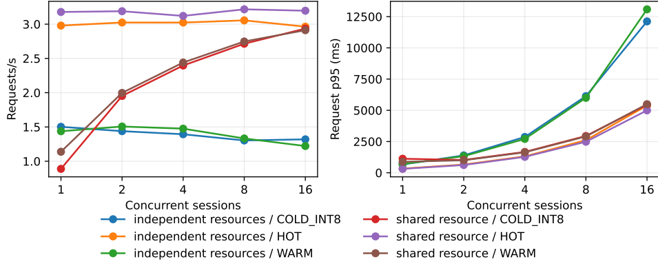
Figure 24: Shared and independent MLX resources through 16 concurrent sessions. The finite waves include promotion and serialized model queueing.
