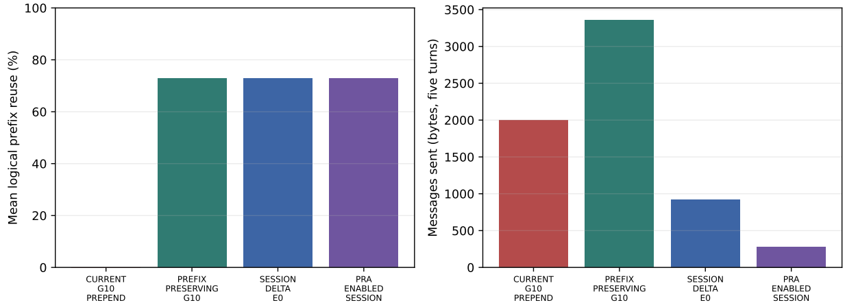
Figure 13: Five-turn deterministic gateway profile. The left panel reports logical reuse of the exact prior serialized message prefix after turn one; the right reports message bytes sent. Resource bytes are reported separately in Table 15.
