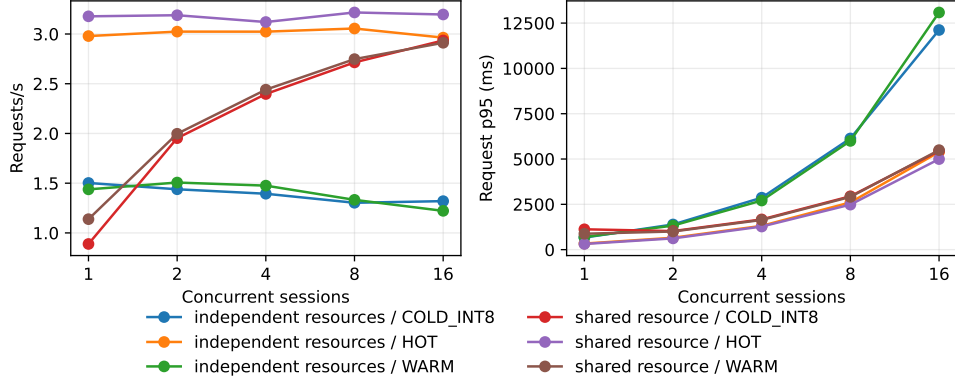
Figure 27: Shared and independent MLX resources through 16 concurrent sessions. The finite waves include promotion and serialized model queueing.
