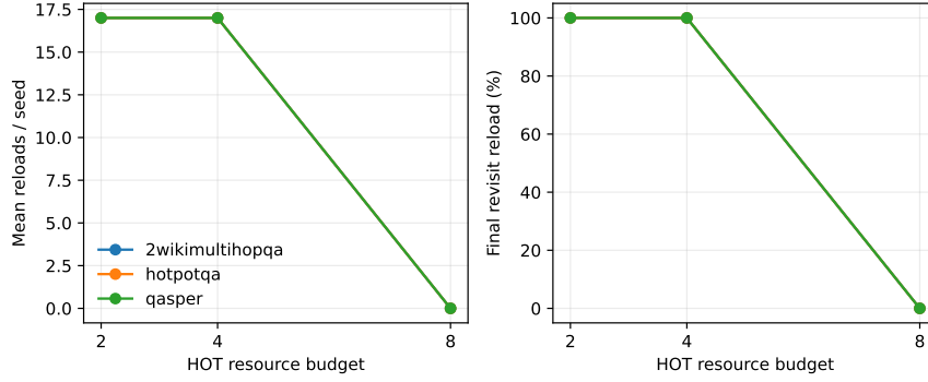
Figure 28: Sustained pressure exposes a working-set threshold rather than a quality effect: once all eight resources fit, reloads disappear.
