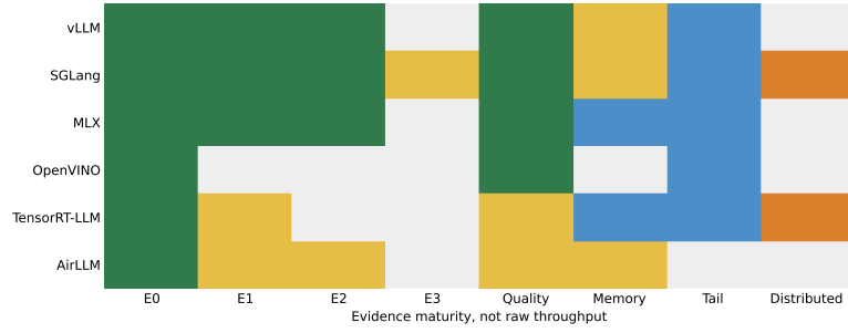
Figure 29: Cross-engine evidence maturity. Darker cells indicate stronger evidence; candidate mechanisms do not automatically promote validated level.
