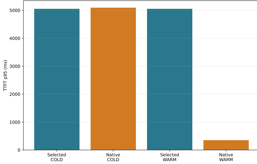
Figure 12: Qwen3-8B selector-frozen TTFT p95 over the same 50 questions. The cold paths remain close; retained native K/V removes repeated selected-text prefill.
