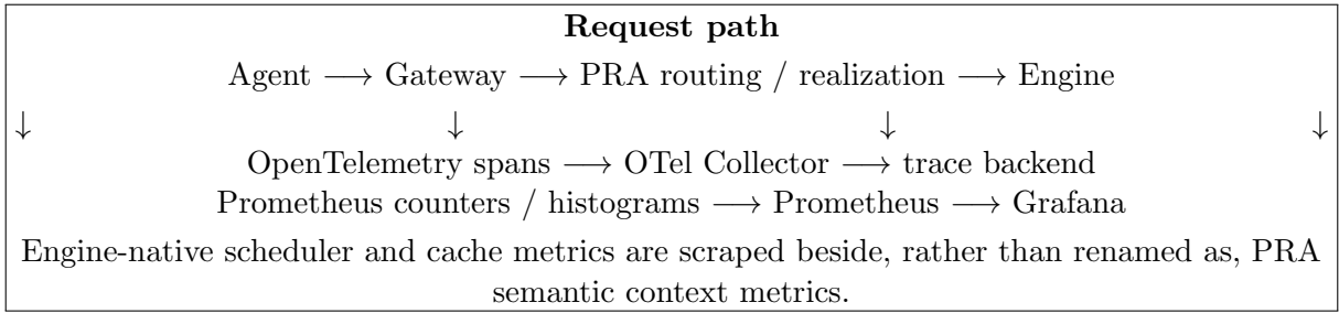
Figure 38: The observability boundary. W3C context joins request causality, while Prometheus and Grafana correlate semantic context decisions with engine-native serving behavior.
