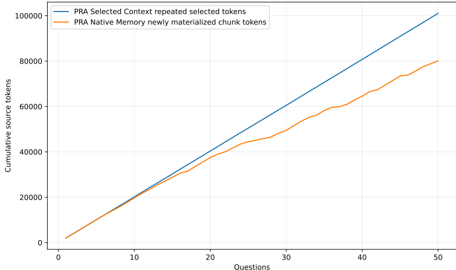
Figure 11: Physical persistent-corpus accounting over 50 changing selections. Chunk-native residency reduces newly encoded source tokens, but this curve must be read with the source-local positional and retained-memory caveats.
