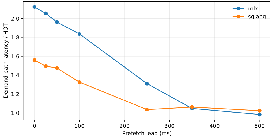
Figure 26: Scheduler-owned WARM promotion can hide request-path stall when useful lead is available. The dashed line is HOT latency.
