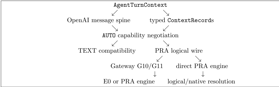
Figure 6: The agent preserves the pretrained conversational spine separately from detached typed context. Compatibility loss occurs only at an explicit TEXT or G10 downgrade; native K/V remains engine-side.
