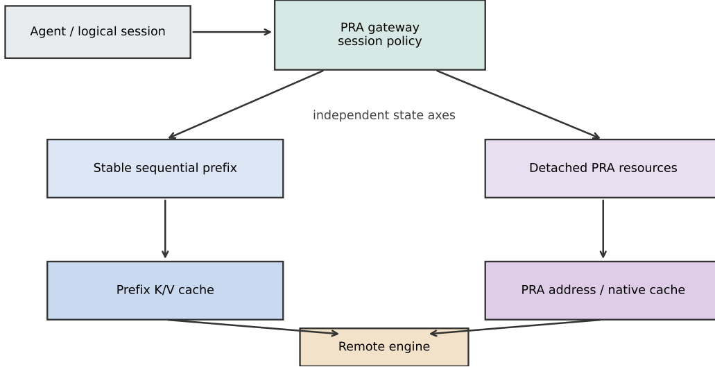
Figure 7: The session-aware gateway maintains two independent state axes. Sequential prompt K/V follows the engine’s ordinary prefix-cache policy; detached PRA resources follow the PRA lifecycle and may be text-materialized at E0 or retained natively at E2+.
