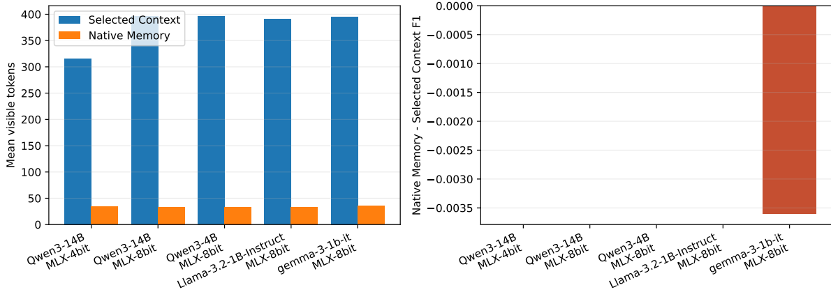
Figure 33: Observed visible-context accounting and Native-Memory-minus-Selected-Context token-F1 change by exact precision encoding. The plot deliberately excludes planned rows; absence is not rendered as zero.
