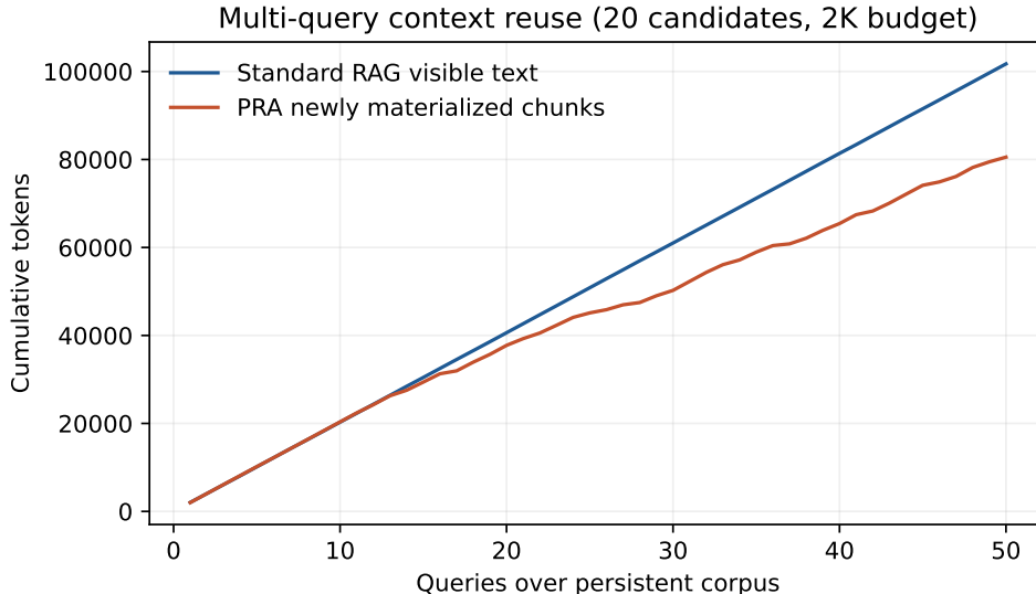
Figure 9: Cumulative selected-text transmission versus unique newly materialized PRA chunks over 50 real-retrieval questions. Physical cache hits and wall time remain for engine qualification.
