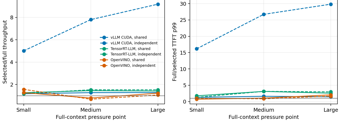
Figure 30: Within-engine throughput and TTFT-tail ratios over three context pressure points. Absolute rates are not compared across dissimilar hardware.
