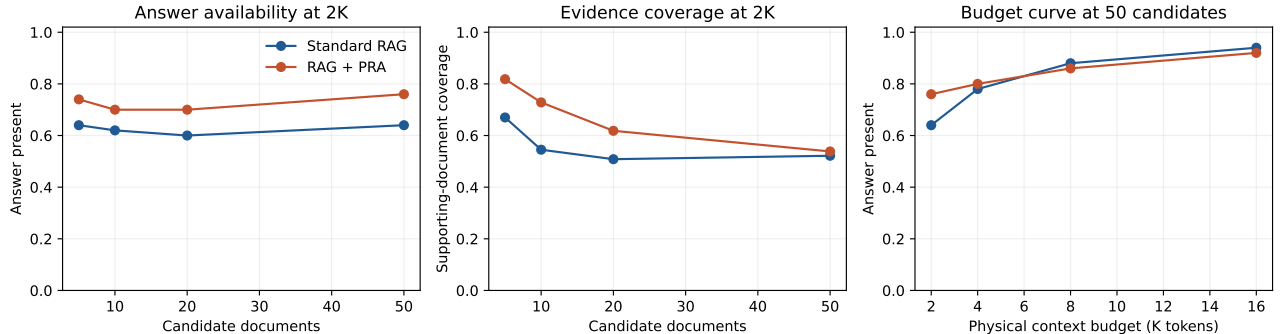
Figure 8: Gold-present candidate and physical-budget curves. Parameter-free PRA has its clearest advantage under the 2K bottleneck; the conditions converge as most useful chunks fit. The vertical quantity is answer availability, not model accuracy.
