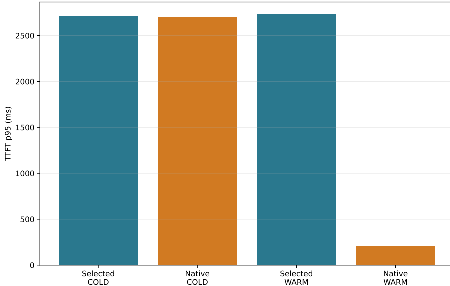
Figure 11: Selector-frozen generic-PRA TTFT p95. Native realization is near the Selected Context control when cold and much faster after retained-K/V reuse; cold and warm measurements are not averaged.
