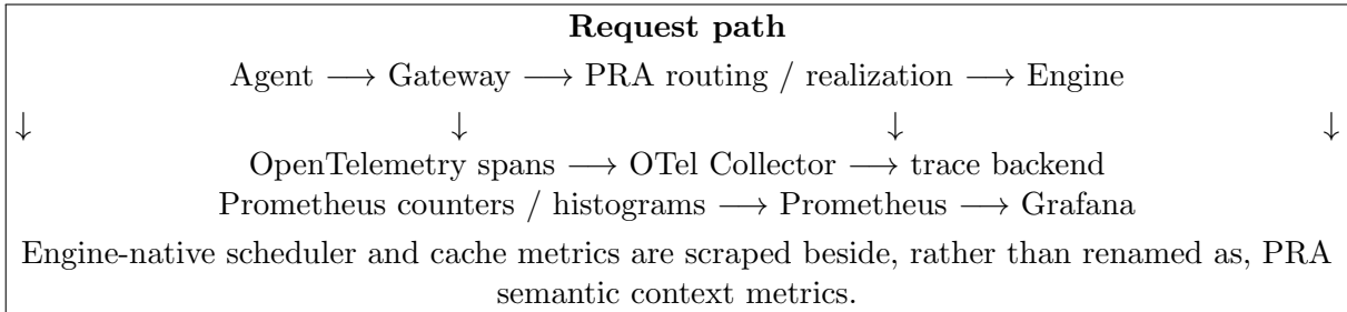
Figure 39: The observability boundary. W3C context joins request causality, while Prometheus and Grafana correlate semantic context decisions with engine-native serving behavior.
