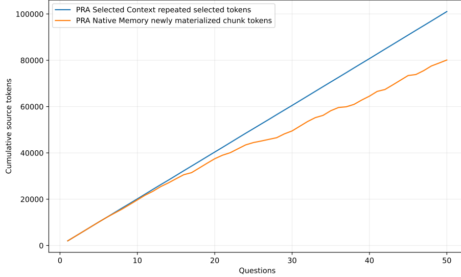
Figure 12: Physical persistent-corpus accounting over 50 changing selections. Chunk-native residency reduces newly encoded source tokens, but this curve must be read with the source-local positional and retained-memory caveats.
