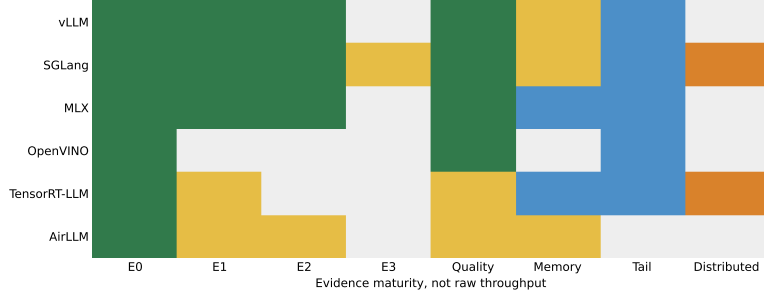
Figure 30: Cross-engine evidence maturity. Darker cells indicate stronger evidence; candidate mechanisms do not automatically promote validated level.
