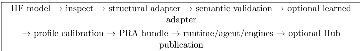
Figure 37: The model-onboarding path. Each arrow is a separately inspectable service boundary rather than an implicit side effect of one CLI callback.
