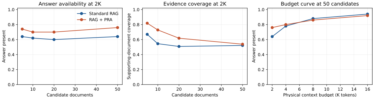
Figure 9: Gold-present candidate and physical-budget curves. Parameter-free PRA has its clearest advantage under the 2K bottleneck; the conditions converge as most useful chunks fit. The vertical quantity is answer availability, not model accuracy.
