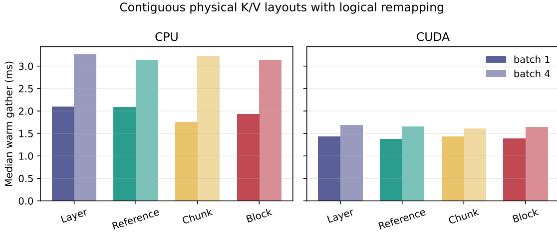
Figure 20: Warm materialization from four physically distinct contiguous stores. Every layout restores the same logical per-layer K/V before attention.
