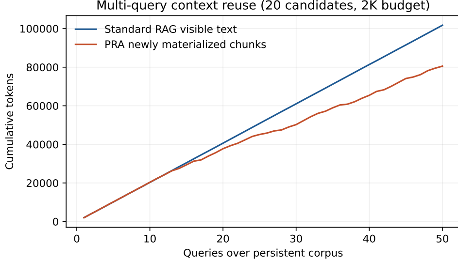
Figure 10: Cumulative selected-text transmission versus unique newly materialized PRA chunks over 50 real-retrieval questions. Physical cache hits and wall time remain for engine qualification.
