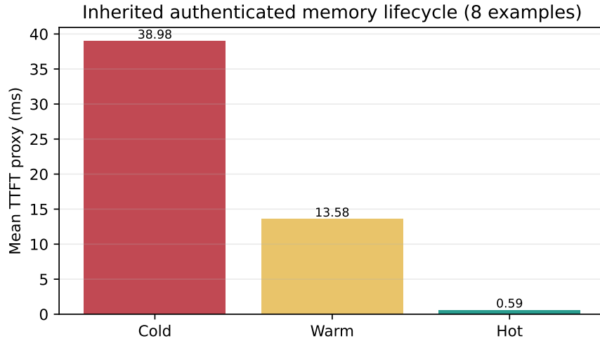
Figure 22: Inherited Paper 4 lifecycle proxy over eight examples. Cold includes fetch and native encoding; warm reuses native encoding; hot reuses selected K/V.
