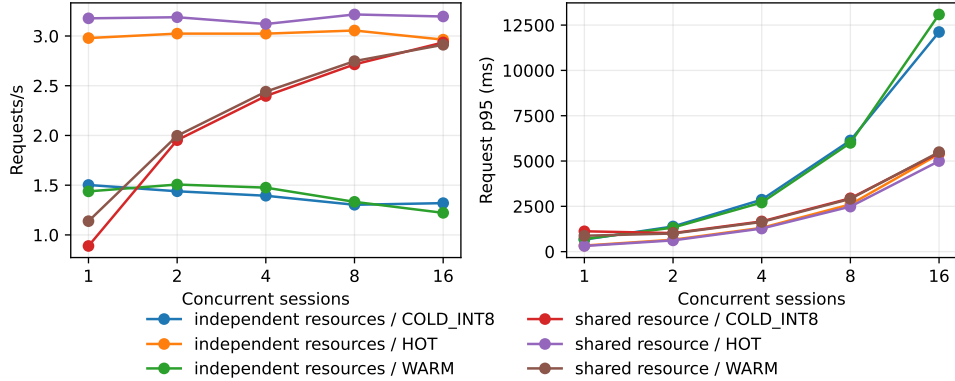
Figure 28: Shared and independent MLX resources through 16 concurrent sessions. The finite waves include promotion and serialized model queueing.
