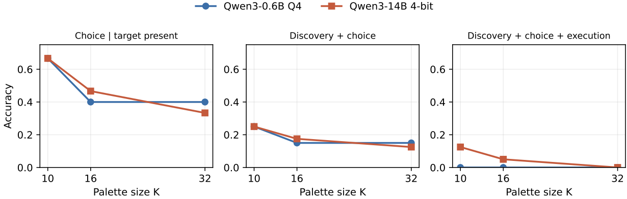
Figure 3: The same 8,192-tool diversity-union palettes evaluated by two frozen Qwen choosers. Discovery recall is fixed at 15/40 for all displayed points. The 14B model modestly improves oracle argument construction but does not produce a monotone discrimination advantage as the palette grows.
