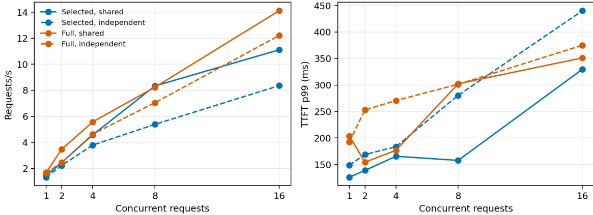
Figure 2: Expanded OpenVINO E0 throughput and TTFT tails through concurrency 16. The full-context request/s lines include wrong, shorter completions and must be read with Table 6.
