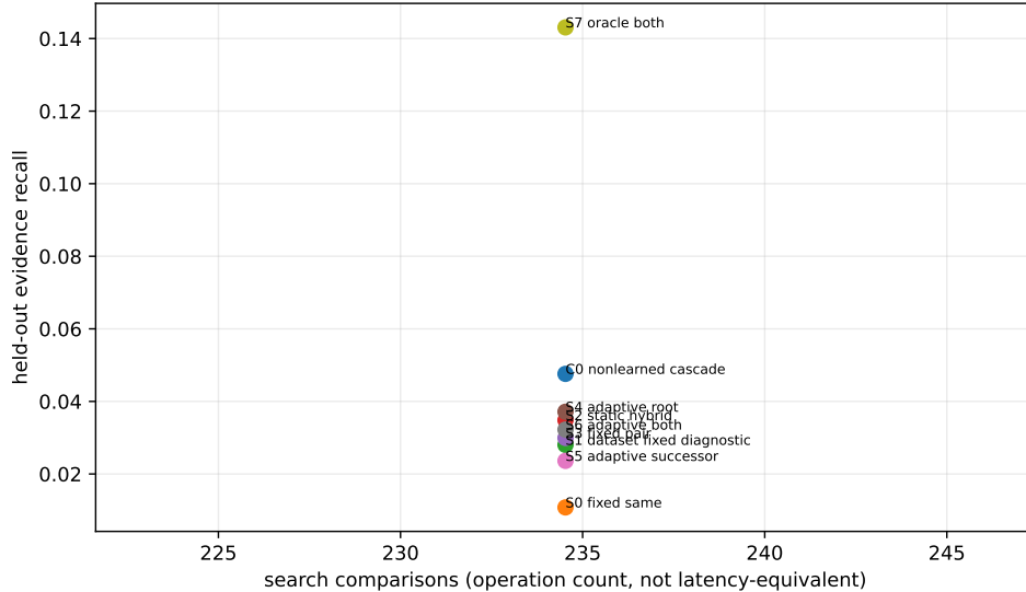
Figure 12: Held-out method policies. The horizontal axis shows search-operation counts and is not a latency-equivalent scalar across semantic GEMM, postings, and token-span work.
