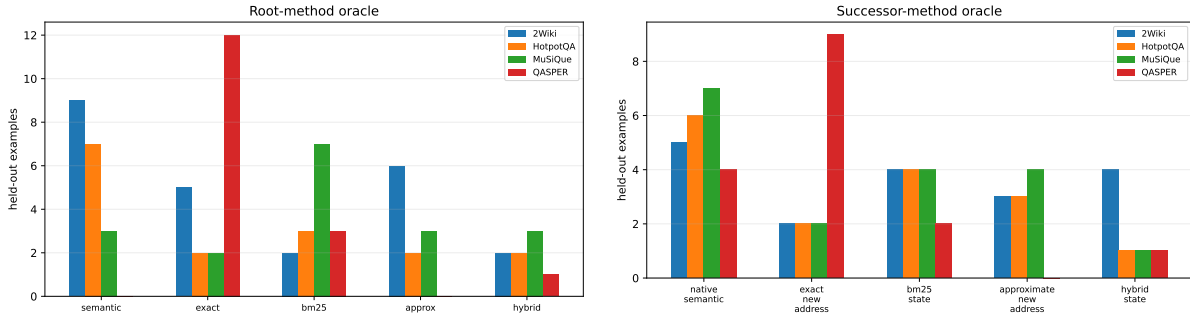
Figure 10: Held-out method-oracle distributions. Root (left) and successor (right) choices are heterogeneous across all four datasets; counts are identities, not repeated model seeds.
