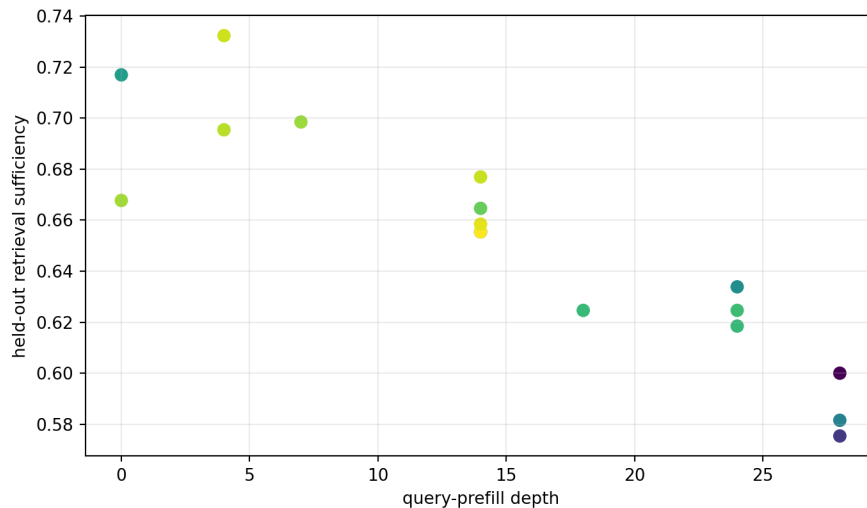
Figure 16: Held-out profile-router quality over query-prefill depth. Color encodes total abstract cost. Greater depth does not produce a monotonic quality gain.
