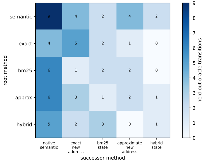
Figure 11: Held-out joint-oracle transitions. Sparse mass across 22 cells argues against tying root and successor representations, but does not say that an observable selector can predict the cell.
