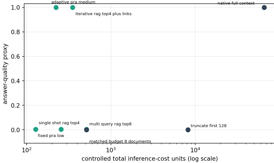
Figure 21: Controlled two-hop quality/cost frontier. Iterative RAG is the appropriate comparison for iterative PRA; a one-shot RAG baseline is insufficient.
