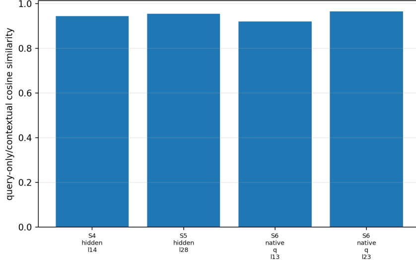
Figure 17: Cosine similarity between pooled query-only and 256-token source-contextualized question states. Contextual processing is expensive, while the selected representations remain close.
