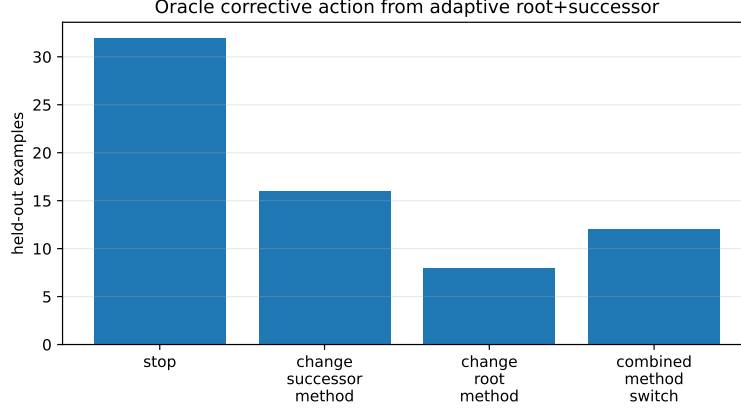
Figure 14: Evaluator-side correction decomposition from adaptive root+successor selection. The learned retry predicts the delta and replacement methods separately; it never receives gold evidence.
