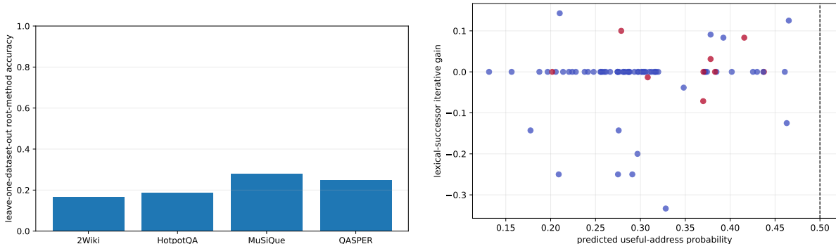
Figure 13: Left: leave-one-dataset-out method accuracy without dataset identity. Right: predicted useful-address probability versus lexical-successor gain; the fitted gate abstains at .5.
