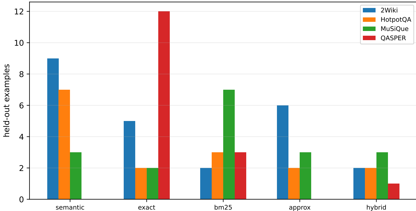
Root-method oracle
