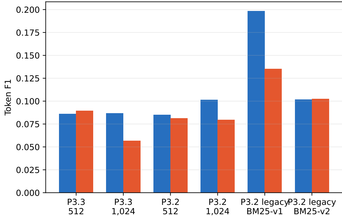
Token overlap
