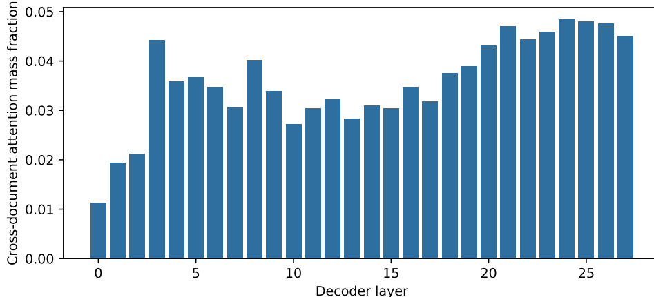
Figure 4: Mean share of packed-teacher cross-document attention mass by decoder layer. Later layers carry more aggregate mass, but no narrow layer band dominates.
