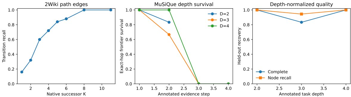
Figure 2: Natural graph diagnostics. 2Wiki exposes transition/path fidelity; MuSiQue separates annotated task depth from minimum native recovery depth.
