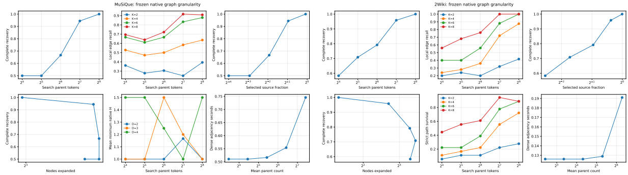
Figure 27: Frozen native graph granularity. Finer nodes reduce selected payload and increase evidence density, but direct edge and complete recovery deteriorate. Dense exact adjacency remains the cold-cost bottleneck; search itself is milliseconds.
