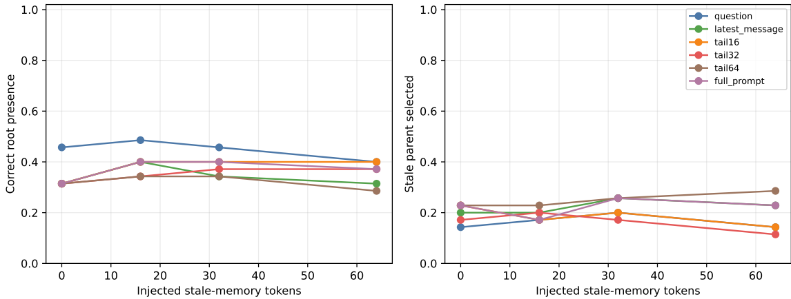
Figure 19: Held-out Hotpot response to injected stale-memory text. Left: current root entry. Right: selection of the explicitly non-oracle stale parent. The validation-frozen latest-message boundary is bounded and cheaper, but stale-context resistance remains mixed on this sample.
