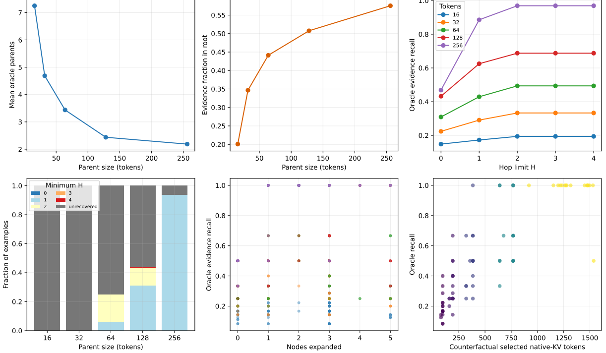
Figure 24: Chunk topology, recovery depth, and the discovery/materialization frontier. The stacked depth panel reports the minimum H under K = 6, B = \text{None} and labels failures explicitly as unrecovered. The other quality panels use the frozen K = 4, B = 6 operating point. Native K/V is not actually materialized; bottom-right token counts are counterfactual payloads for the visited parents.
