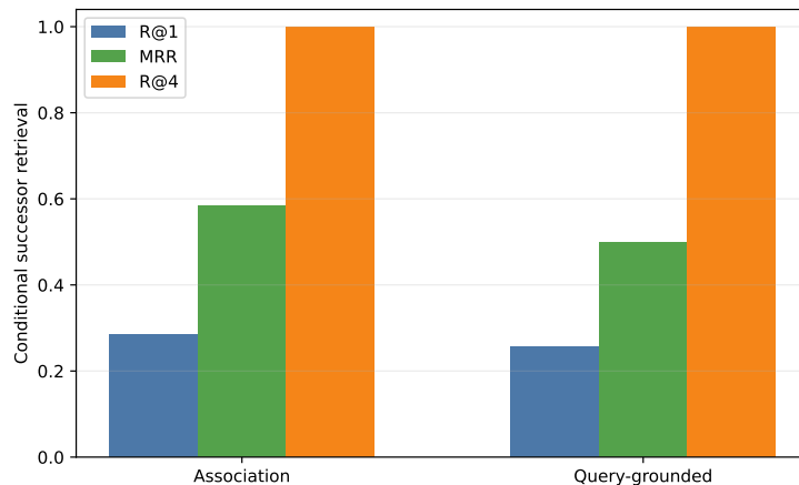
Figure 20: Held-out conditional successor retrieval. Static current-query facets preserve Top-4 availability but worsen the order inside that bounded candidate set.
