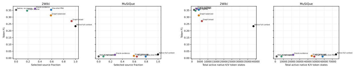
Figure 6: Answer F1 versus conceptual selected source (left) and actual peak native K/V state (right). Higher recovery does not produce a monotone output frontier.
