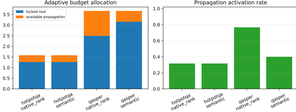
Figure 15: Held-out exploratory budget allocation and propagation activation at 20%. The final parent budget remains matched even when the locally selected lock count differs.
