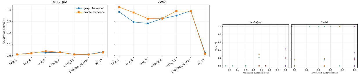
Figure 7: Left: fixed evidence under different consumption bands. All-layer injection collapses 2Wiki output. Right: annotated-evidence recall is not sufficient for answer quality.
