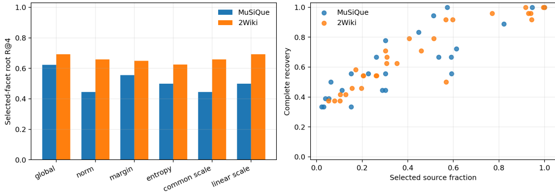
Figure 5: Left: executable facet selectors remain below the oracle root-view ceiling. Right: high complete recovery requires broad conceptual source activation.
